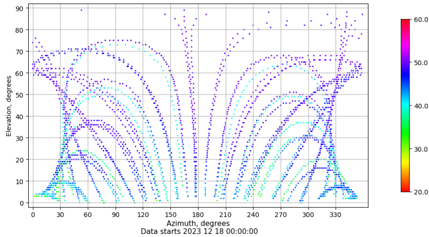
Azimuth-elevation plot for station RIO1. Signal to Noise S1C Data file RIO100ESP_R_2023352.xtr
