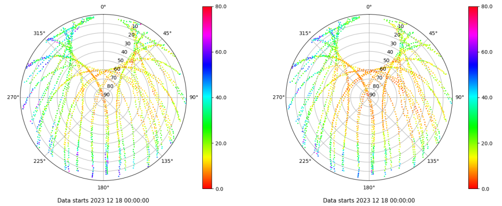
Skyplot for station RIO1. Parameter M1C Data file RIO100ESP_R_2023352.xtr Skyplot for station RIO1. Parameter M2P Data file RIO100ESP_R_2023352.xtr
