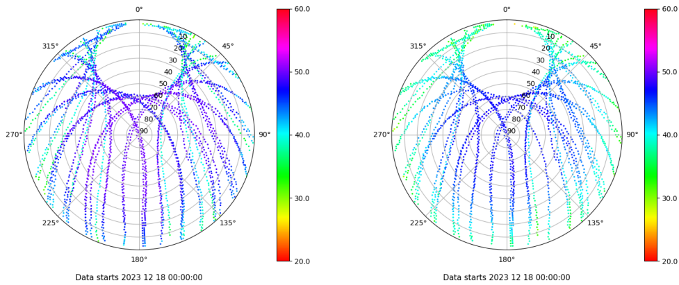
Skyplot for station RIO1. Signal to Noise S1C Data file RIO100ESP_R_2023352.xtr Skyplot for station RIO1. Signal to Noise S2P Data file RIO100ESP_R_2023352.xtr
