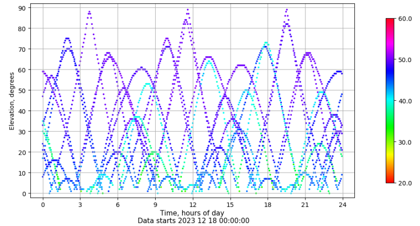
Time-elevation plot for station RIO1. Signal to Noise S1C Data file RIO100ESP_R_2023352.xtr
