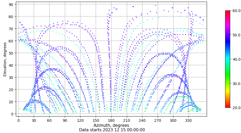
Azimuth-elevation plot for station RIO1. Signal to Noise S1C Data file RIO100ESP_R_2023349.xtr
