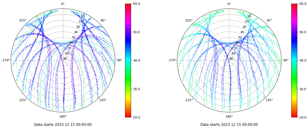
Skyplot for station RIO1. Signal to Noise S1C Data file RIO100ESP_R_2023349.xtr Skyplot for station RIO1. Signal to Noise S2P Data file RIO100ESP_R_2023349.xtr
