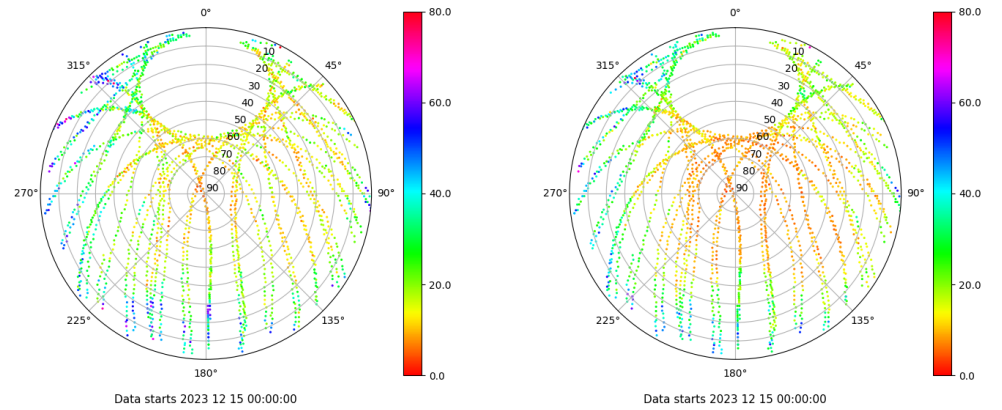
Skyplot for station RIO1. Parameter M1C Data file RIO100ESP_R_2023349.xtr Skyplot for station RIO1. Parameter M2P Data file RIO100ESP_R_2023349.xtr
