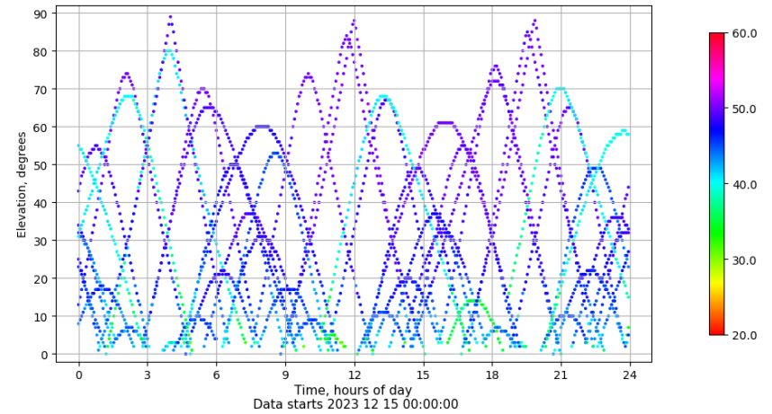
Time-elevation plot for station RIO1. Signal to Noise S1C Data file RIO100ESP_R_2023349.xtr
