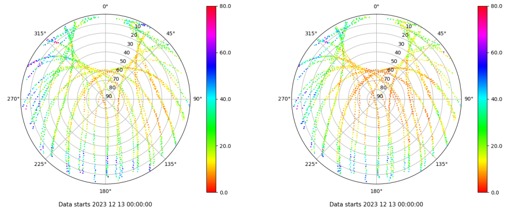
Skyplot for station RIO1. Parameter M1C Data file RIO100ESP_R_2023347.xtr Skyplot for station RIO1. Parameter M2P Data file RIO100ESP_R_2023347.xtr
