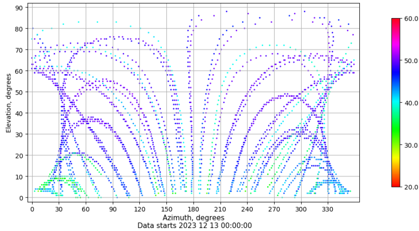
Azimuth-elevation plot for station RIO1. Signal to Noise S1C Data file RIO100ESP_R_2023347.xtr
