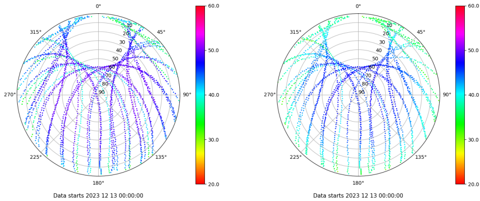
Skyplot for station RIO1. Signal to Noise S1C Data file RIO100ESP_R_2023347.xtr Skyplot for station RIO1. Signal to Noise S2P Data file RIO100ESP_R_2023347.xtr
