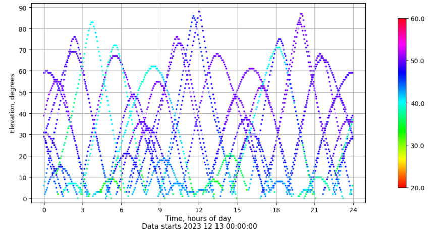
Time-elevation plot for station RIO1. Signal to Noise S1C Data file RIO100ESP_R_2023347.xtr
