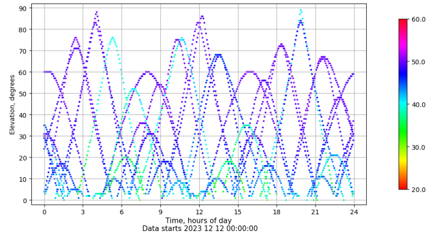
Time-elevation plot for station RIO1. Signal to Noise S1C Data file RIO100ESP_R_2023346.xtr
