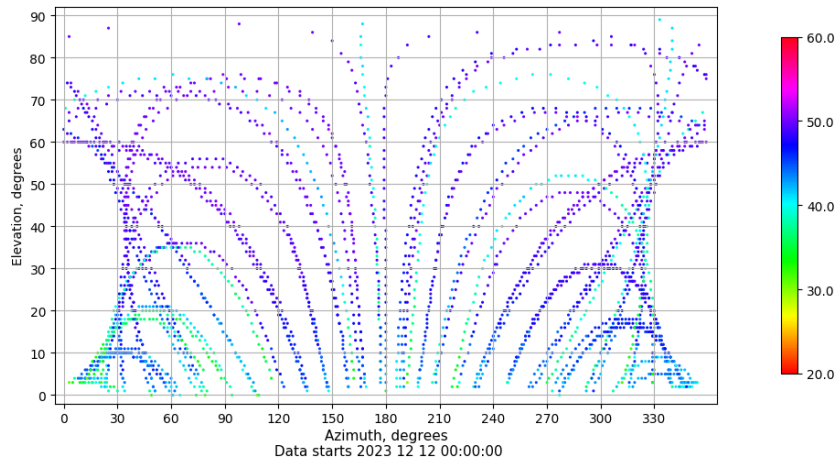
Azimuth-elevation plot for station RIO1. Signal to Noise S1C Data file RIO100ESP_R_2023346.xtr
