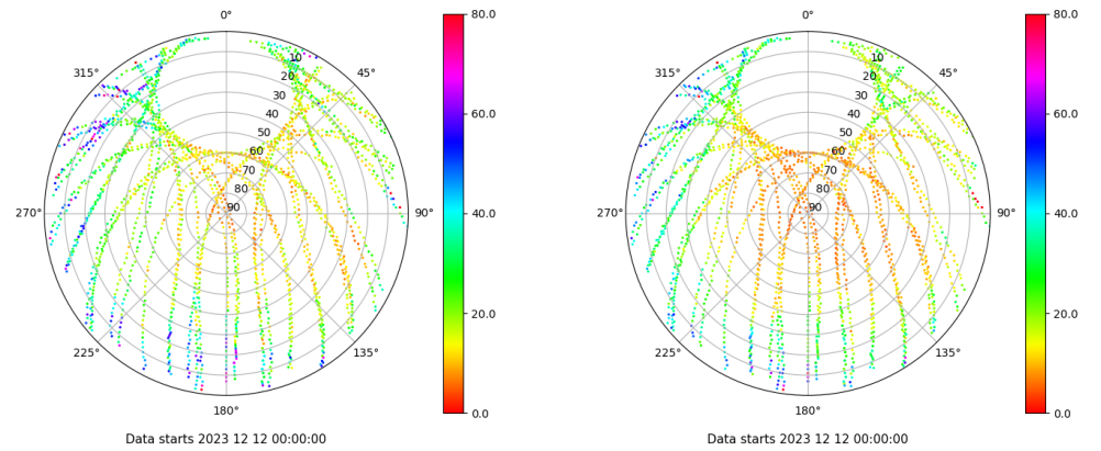
Skyplot for station RIO1. Parameter M1C Data file RIO100ESP_R_2023346.xtr Skyplot for station RIO1. Parameter M2P Data file RIO100ESP_R_2023346.xtr
