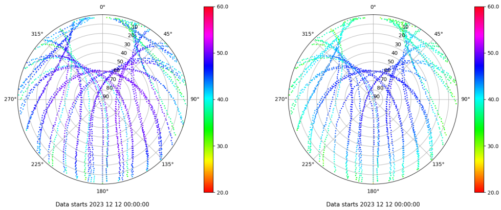
Skyplot for station RIO1. Signal to Noise S1C Data file RIO100ESP_R_2023346.xtr Skyplot for station RIO1. Signal to Noise S2P Data file RIO100ESP_R_2023346.xtr
