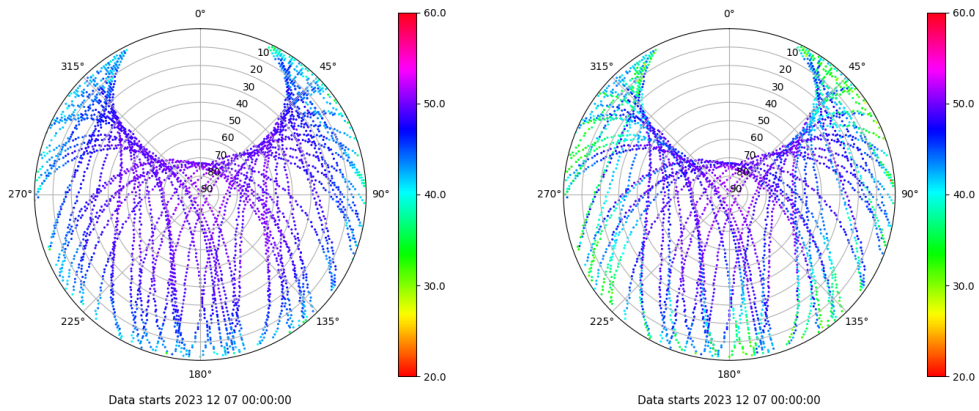
Skyplot for station RIO1. Signal to Noise S1C Data file RIO100ESP_R_2023341.xtr Skyplot for station RIO1. Signal to Noise S2W Data file RIO100ESP_R_2023341.xtr
