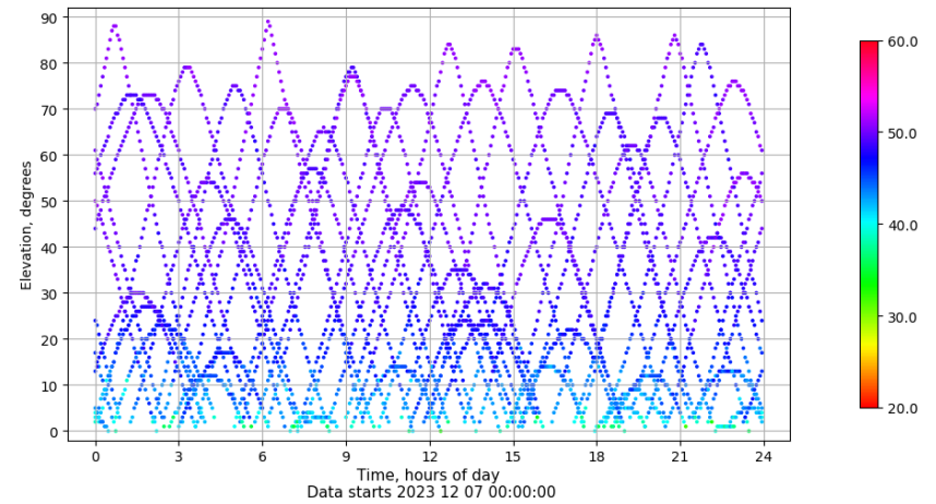
Time-elevation plot for station RIO1. Signal to Noise S1C Data file RIO100ESP_R_2023341.xtr
