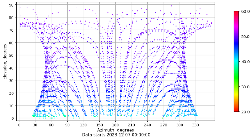
Azimuth-elevation plot for station RIO1. Signal to Noise S1C Data file RIO100ESP_R_2023341.xtr
