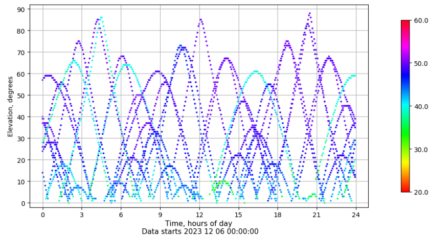
Time-elevation plot for station RIO1. Signal to Noise S1C Data file RIO100ESP_R_2023340.xtr
