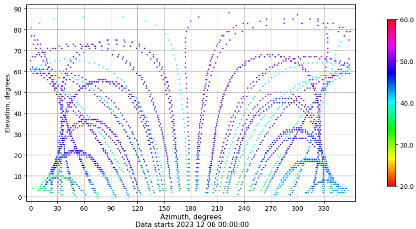
Azimuth-elevation plot for station RIO1. Signal to Noise S1C Data file RIO100ESP_R_2023340.xtr
