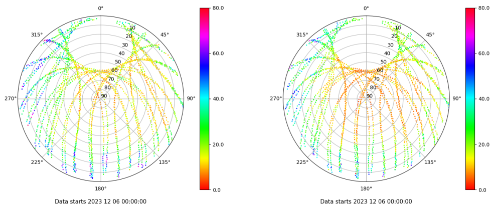
Skyplot for station RIO1. Parameter M1C Data file RIO100ESP_R_2023340.xtr Skyplot for station RIO1. Parameter M2P Data file RIO100ESP_R_2023340.xtr
