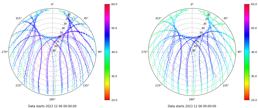
Skyplot for station RIO1. Signal to Noise S1C Data file RIO100ESP_R_2023340.xtr Skyplot for station RIO1. Signal to Noise S2P Data file RIO100ESP_R_2023340.xtr
