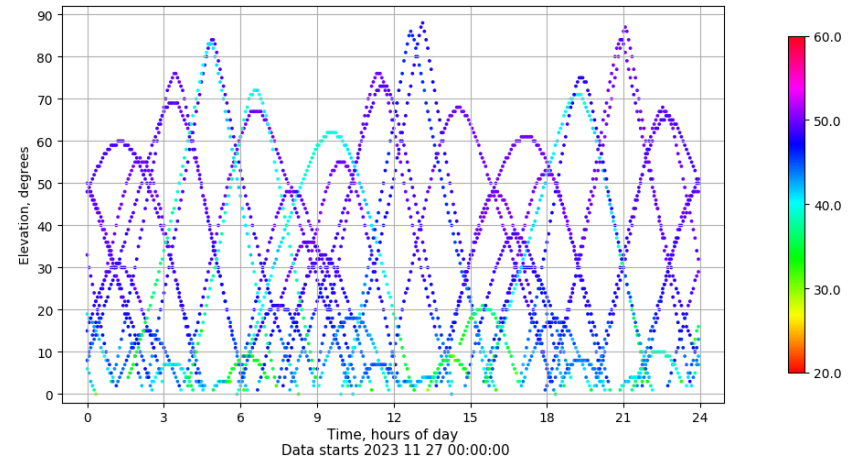
Time-elevation plot for station RIO1. Signal to Noise S1C Data file RIO100ESP_R_2023331.xtr
