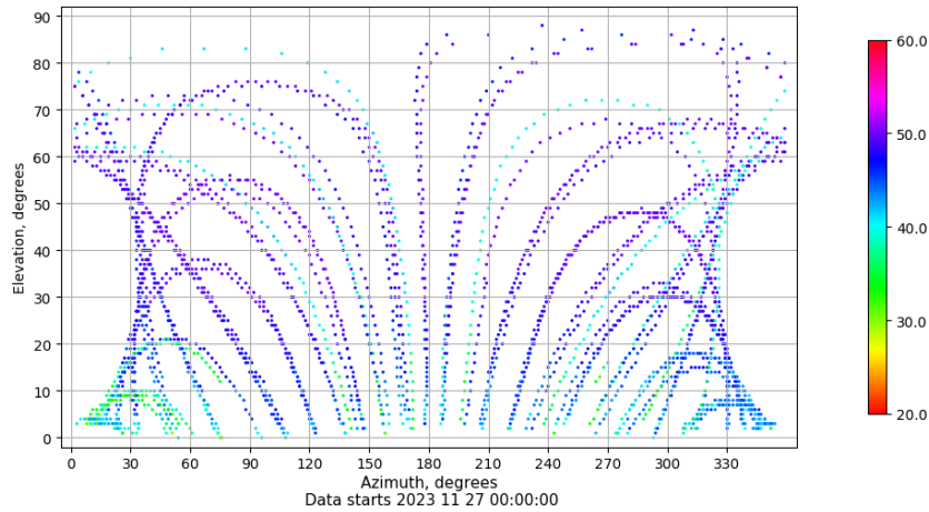
Azimuth-elevation plot for station RIO1. Signal to Noise S1C Data file RIO100ESP_R_2023331.xtr
