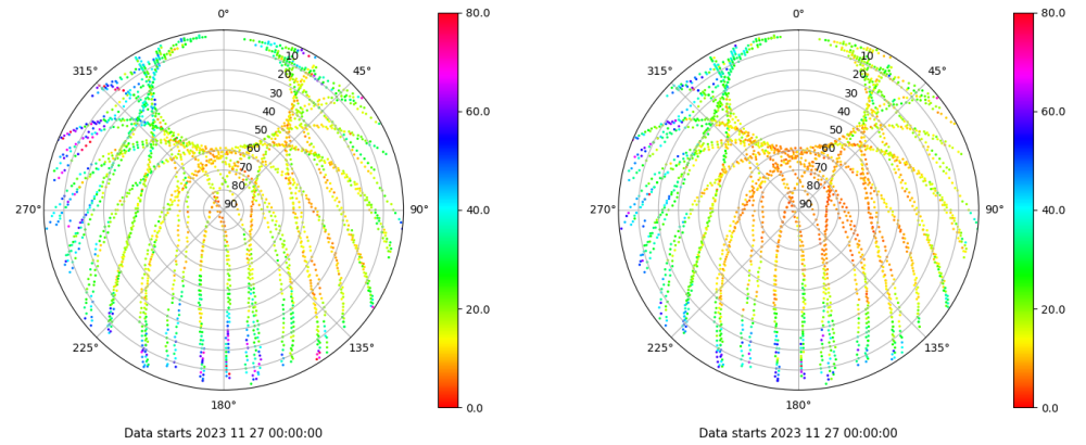
Skyplot for station RIO1. Parameter M1C Data file RIO100ESP_R_2023331.xtr Skyplot for station RIO1. Parameter M2P Data file RIO100ESP_R_2023331.xtr
