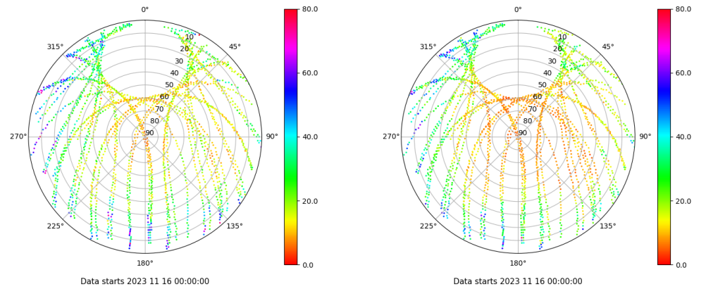
Skyplot for station RIO1. Parameter M1C Data file RIO100ESP_R_2023320.xtr Skyplot for station RIO1. Parameter M2P Data file RIO100ESP_R_2023320.xtr
