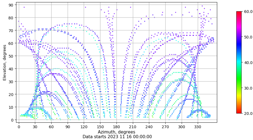
Azimuth-elevation plot for station RIO1. Signal to Noise S1C Data file RIO100ESP_R_2023320.xtr
