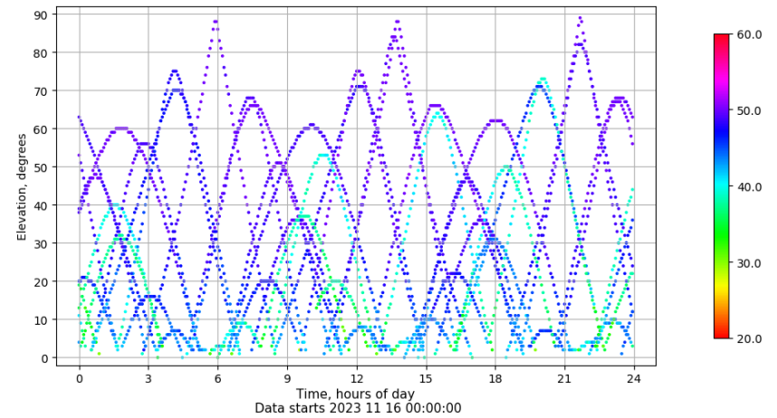
Time-elevation plot for station RIO1. Signal to Noise S1C Data file RIO100ESP_R_2023320.xtr
