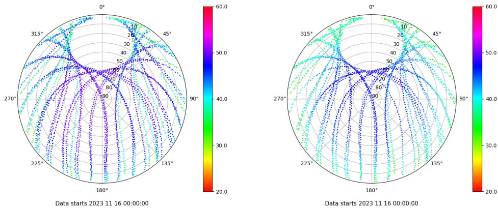
Skyplot for station RIO1. Signal to Noise S1C Data file RIO100ESP_R_2023320.xtr Skyplot for station RIO1. Signal to Noise S2P Data file RIO100ESP_R_2023320.xtr
