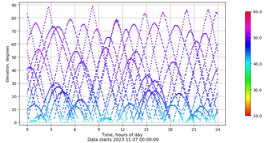
Time-elevation plot for station RIO1. Signal to Noise S1C Data file RIO100ESP_R_2023311.xtr
