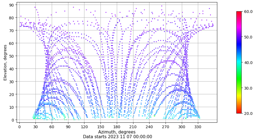
Azimuth-elevation plot for station RIO1. Signal to Noise S1C Data file RIO100ESP_R_2023311.xtr
