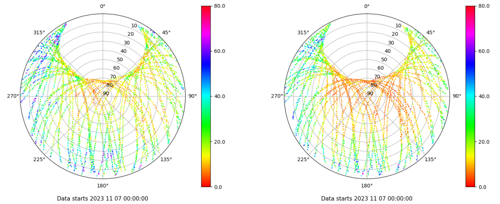
Skyplot for station RIO1. Parameter M1C Data file RIO100ESP_R_2023311.xtr Skyplot for station RIO1. Parameter M2W Data file RIO100ESP_R_2023311.xtr
