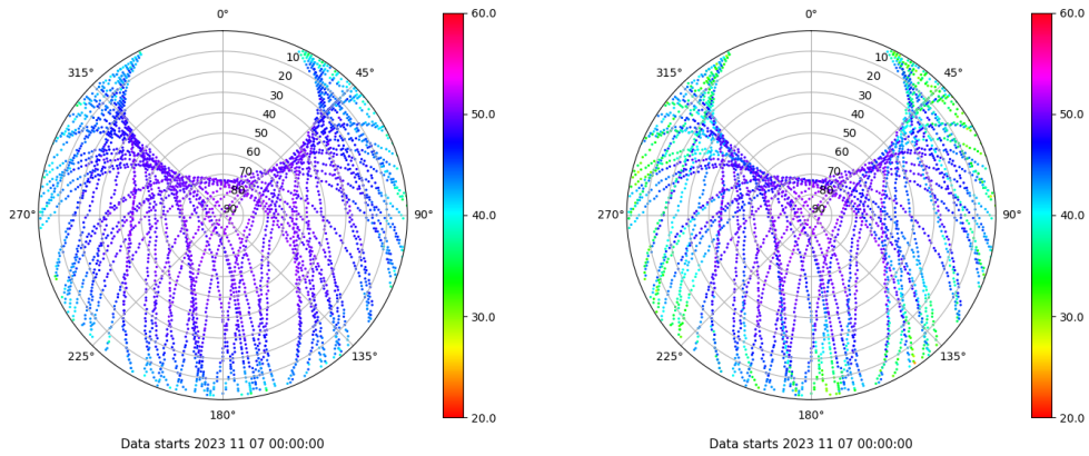
Skyplot for station RIO1. Signal to Noise S1C Data file RIO100ESP_R_2023311.xtr Skyplot for station RIO1. Signal to Noise S2W Data file RIO100ESP_R_2023311.xtr
