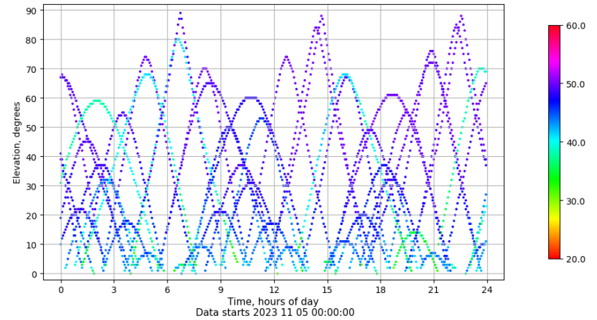
Time-elevation plot for station RIO1. Signal to Noise S1C Data file RIO100ESP_R_2023309.xtr
