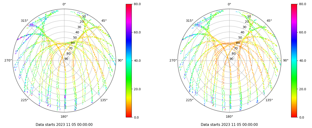
Skyplot for station RIO1. Parameter M1C Data file RIO100ESP_R_2023309.xtr Skyplot for station RIO1. Parameter M2P Data file RIO100ESP_R_2023309.xtr
