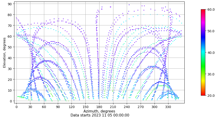
Azimuth-elevation plot for station RIO1. Signal to Noise S1C Data file RIO100ESP_R_2023309.xtr
