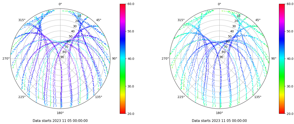
Skyplot for station RIO1. Signal to Noise S1C Data file RIO100ESP_R_2023309.xtr Skyplot for station RIO1. Signal to Noise S2P Data file RIO100ESP_R_2023309.xtr
