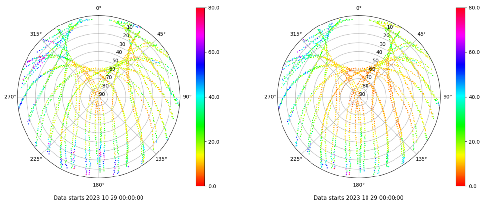
Skyplot for station RIO1. Parameter M1C Data file RIO100ESP_R_2023302.xtr Skyplot for station RIO1. Parameter M2P Data file RIO100ESP_R_2023302.xtr
