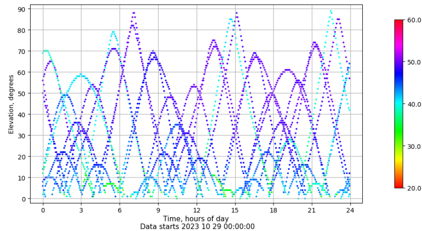
Time-elevation plot for station RIO1. Signal to Noise S1C Data file RIO100ESP_R_2023302.xtr
