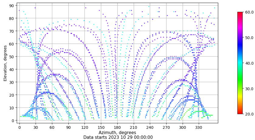
Azimuth-elevation plot for station RIO1. Signal to Noise S1C Data file RIO100ESP_R_2023302.xtr
