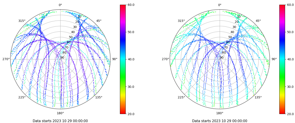
Skyplot for station RIO1. Signal to Noise S1C Data file RIO100ESP_R_2023302.xtr Skyplot for station RIO1. Signal to Noise S2P Data file RIO100ESP_R_2023302.xtr
