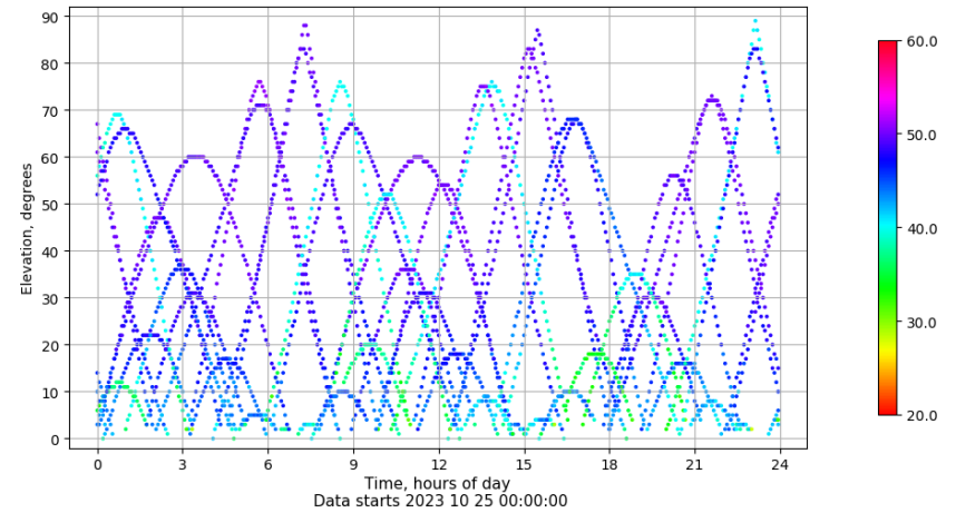
Time-elevation plot for station RIO1. Signal to Noise S1C Data file RIO100ESP_R_2023298.xtr
