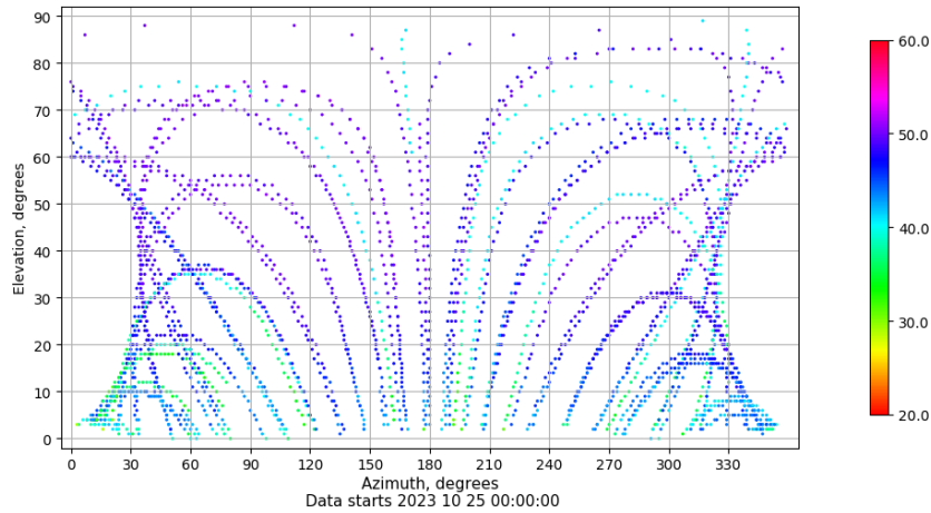
Azimuth-elevation plot for station RIO1. Signal to Noise S1C Data file RIO100ESP_R_2023298.xtr
