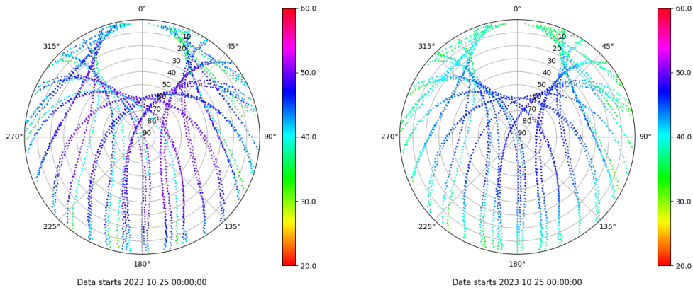
Skyplot for station RIO1. Signal to Noise S1C Data file RIO100ESP_R_2023298.xtr Skyplot for station RIO1. Signal to Noise S2P Data file RIO100ESP_R_2023298.xtr
