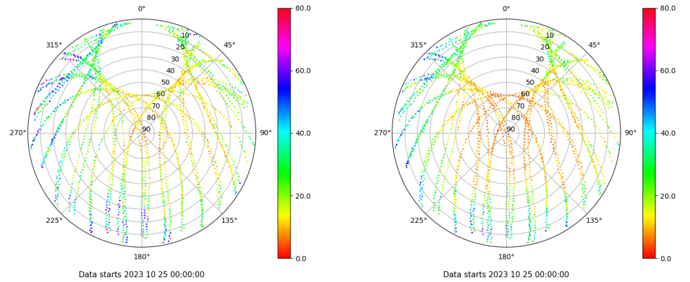
Skyplot for station RIO1. Parameter M1C Data file RIO100ESP_R_2023298.xtr Skyplot for station RIO1. Parameter M2P Data file RIO100ESP_R_2023298.xtr
