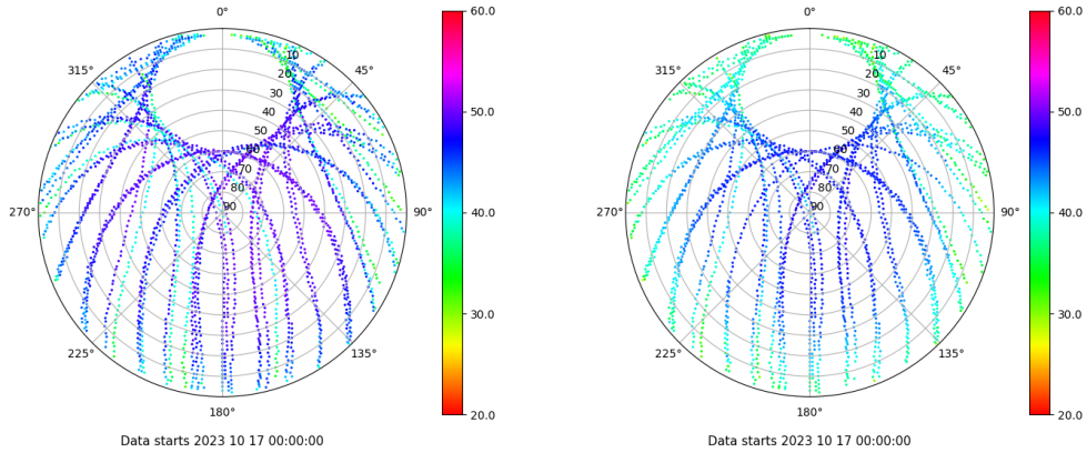
Skyplot for station RIO1. Signal to Noise S1C Data file RIO100ESP_R_2023290.xtr Skyplot for station RIO1. Signal to Noise S2P Data file RIO100ESP_R_2023290.xtr
