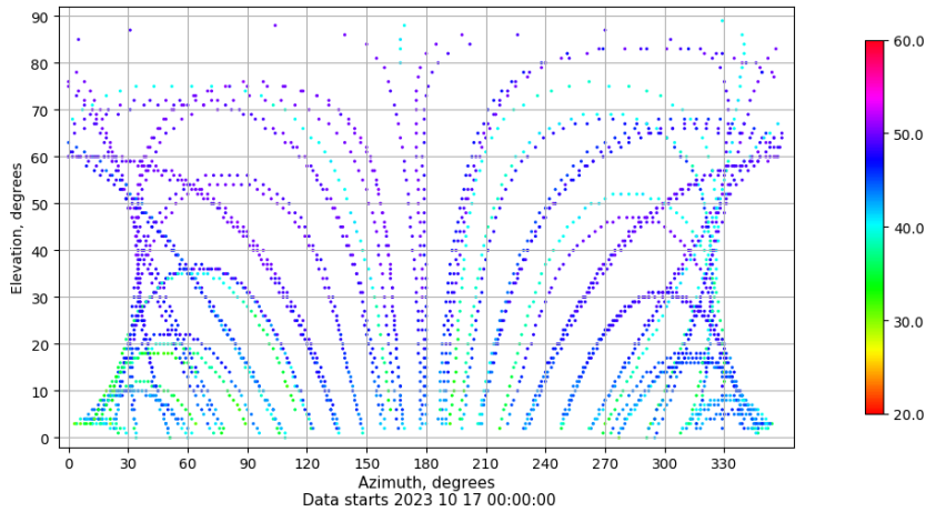
Azimuth-elevation plot for station RIO1. Signal to Noise S1C Data file RIO100ESP_R_2023290.xtr
