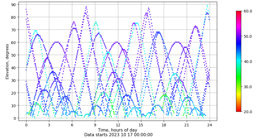
Time-elevation plot for station RIO1. Signal to Noise S1C Data file RIO100ESP_R_2023290.xtr
