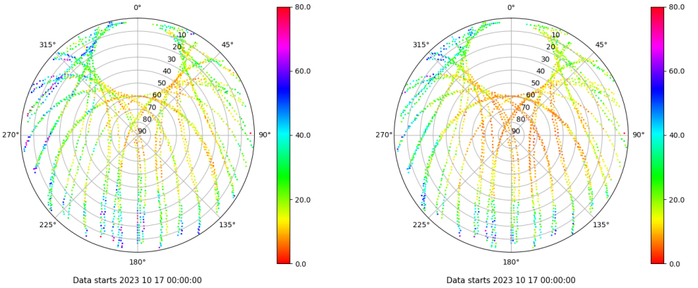
Skyplot for station RIO1. Parameter M1C Data file RIO100ESP_R_2023290.xtr Skyplot for station RIO1. Parameter M2P Data file RIO100ESP_R_2023290.xtr
