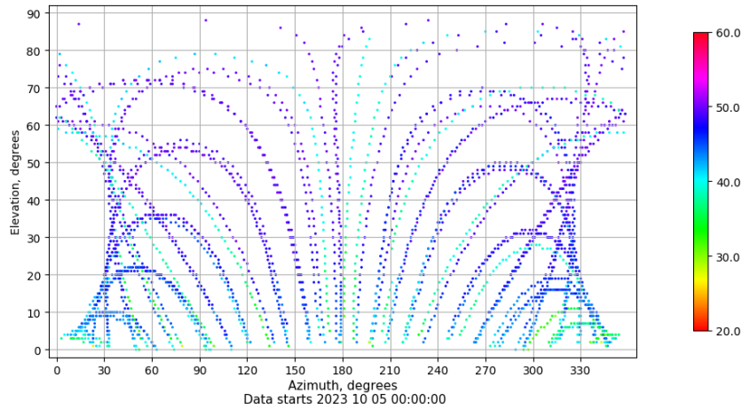
Azimuth-elevation plot for station RIO1. Signal to Noise S1C Data file RIO100ESP_R_2023278.xtr
