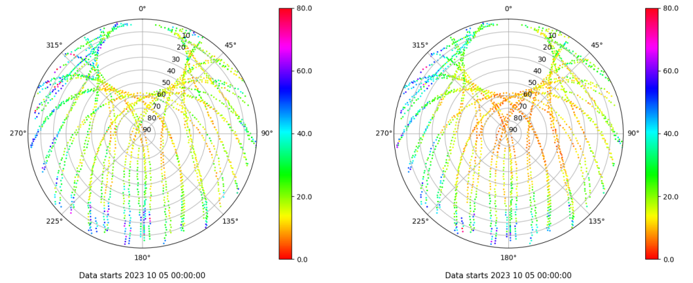
Skyplot for station RIO1. Parameter M1C Data file RIO100ESP_R_2023278.xtr Skyplot for station RIO1. Parameter M2P Data file RIO100ESP_R_2023278.xtr
