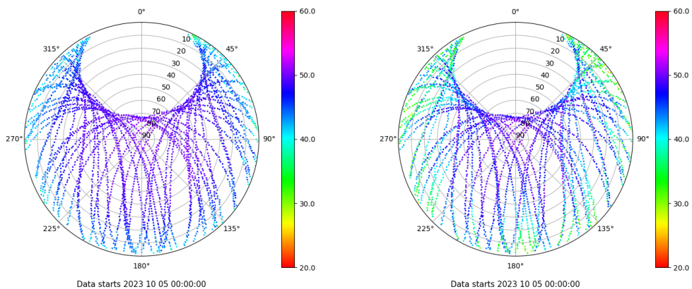
Skyplot for station RIO1. Signal to Noise S1C Data file RIO100ESP_R_2023278.xtr Skyplot for station RIO1. Signal to Noise S2W Data file RIO100ESP_R_2023278.xtr
