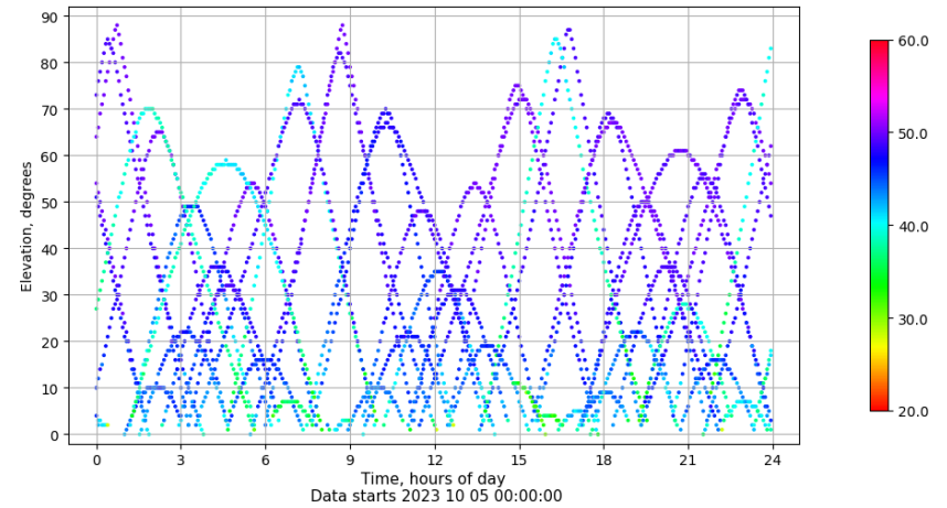
Time-elevation plot for station RIO1. Signal to Noise S1C Data file RIO100ESP_R_2023278.xtr
