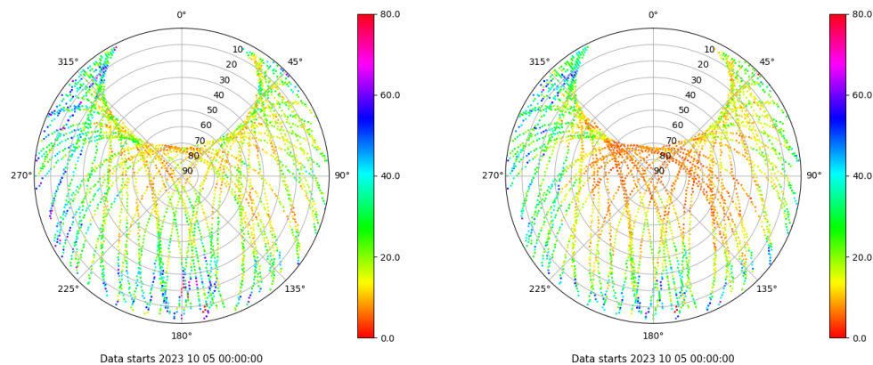
Skyplot for station RIO1. Parameter M1C Data file RIO100ESP_R_2023278.xtr Skyplot for station RIO1. Parameter M2W Data file RIO100ESP_R_2023278.xtr
