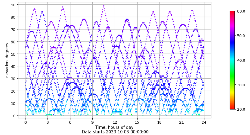
Time-elevation plot for station RIO1. Signal to Noise S1C Data file RIO100ESP_R_2023276.xtr
