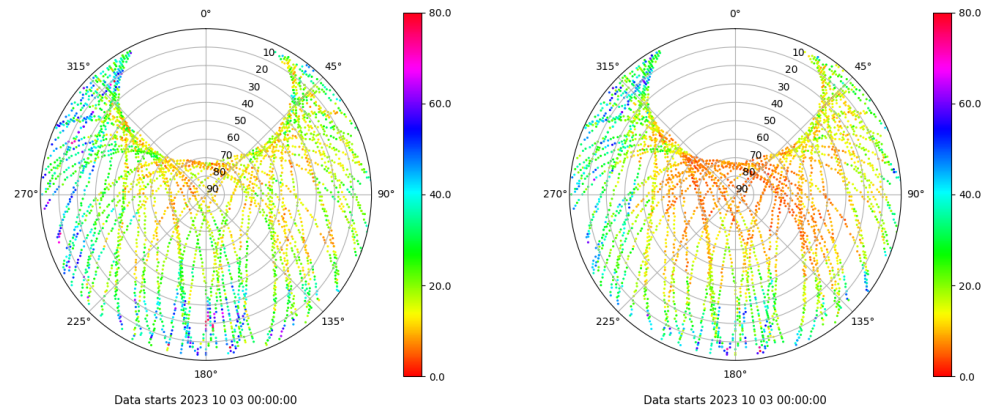
Skyplot for station RIO1. Parameter M1C Data file RIO100ESP_R_2023276.xtr Skyplot for station RIO1. Parameter M2W Data file RIO100ESP_R_2023276.xtr
