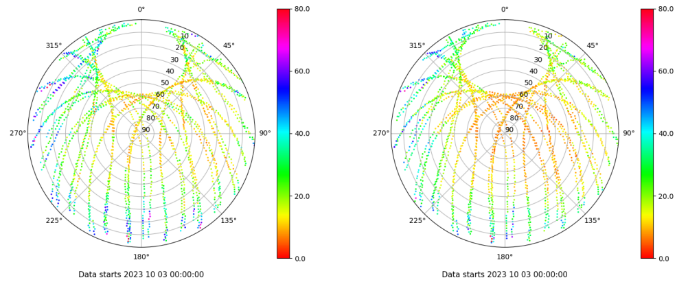
Skyplot for station RIO1. Parameter M1C Data file RIO100ESP_R_2023276.xtr Skyplot for station RIO1. Parameter M2P Data file RIO100ESP_R_2023276.xtr
