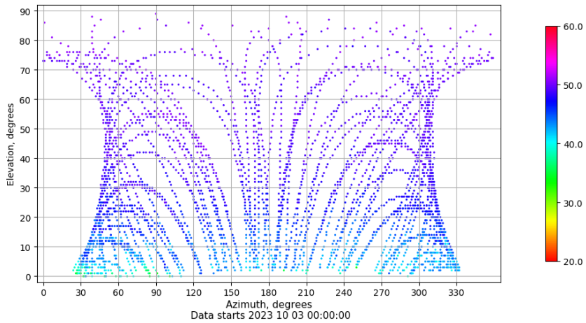
Azimuth-elevation plot for station RIO1. Signal to Noise S1C Data file RIO100ESP_R_2023276.xtr
