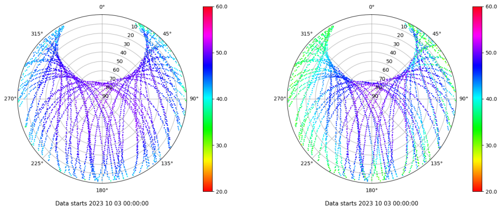
Skyplot for station RIO1. Signal to Noise S1C Data file RIO100ESP_R_2023276.xtr Skyplot for station RIO1. Signal to Noise S2W Data file RIO100ESP_R_2023276.xtr
