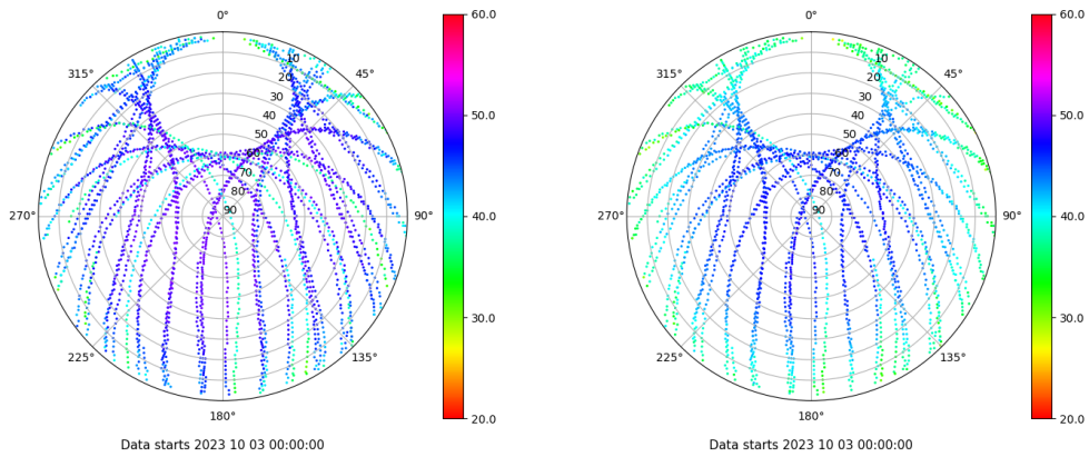
Skyplot for station RIO1. Signal to Noise S1C Data file RIO100ESP_R_2023276.xtr Skyplot for station RIO1. Signal to Noise S2P Data file RIO100ESP_R_2023276.xtr
