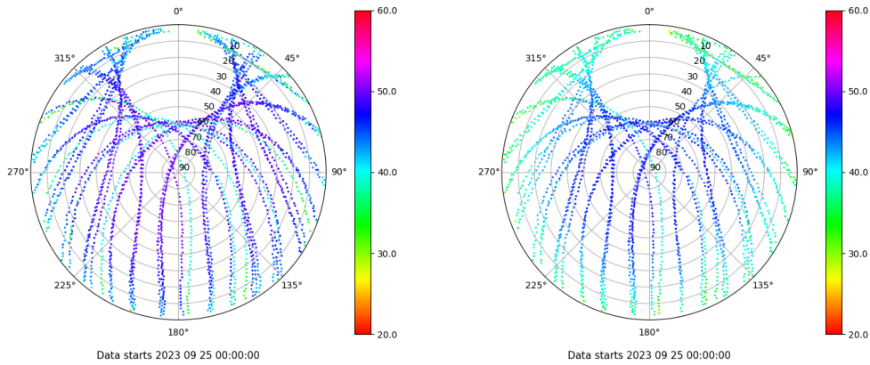
Skyplot for station RIO1. Signal to Noise S1C Data file RIO100ESP_R_2023268.xtr Skyplot for station RIO1. Signal to Noise S2P Data file RIO100ESP_R_2023268.xtr
