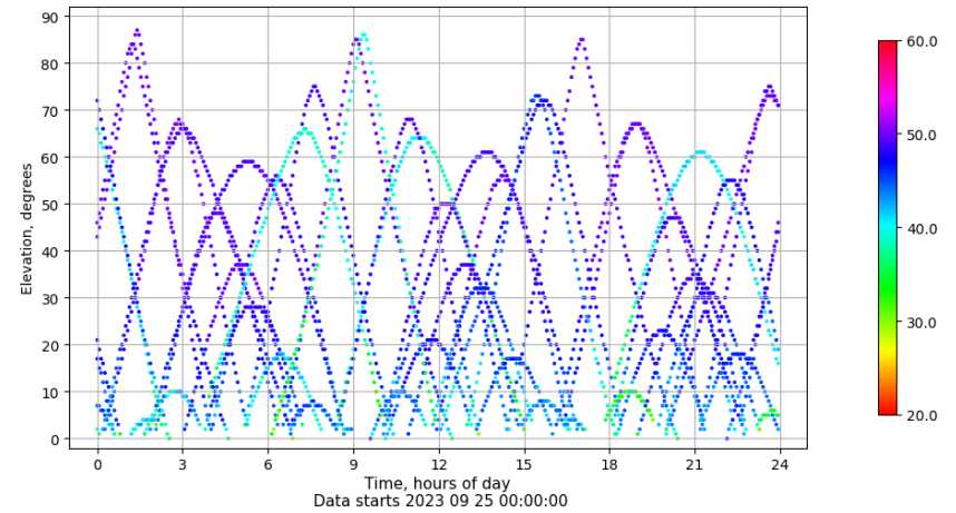
Time-elevation plot for station RIO1. Signal to Noise S1C Data file RIO100ESP_R_2023268.xtr
