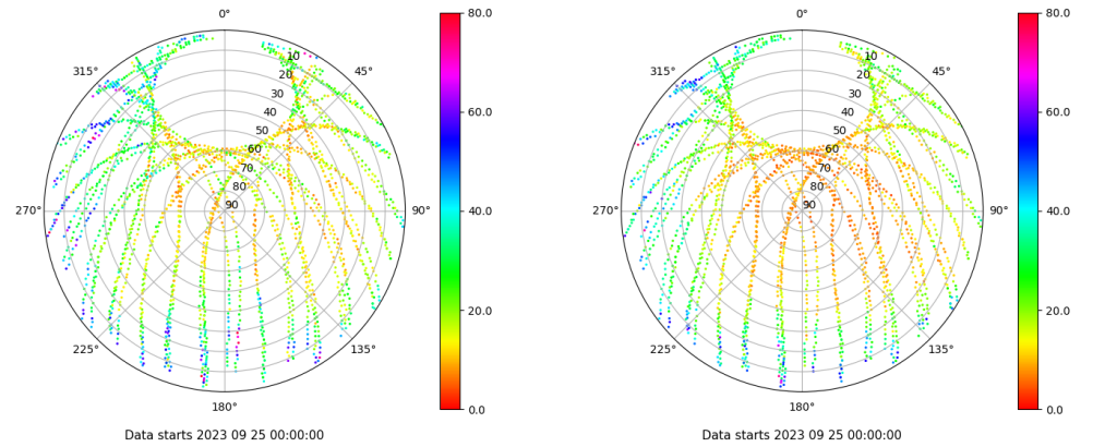
Skyplot for station RIO1. Parameter M1C Data file RIO100ESP_R_2023268.xtr Skyplot for station RIO1. Parameter M2P Data file RIO100ESP_R_2023268.xtr
