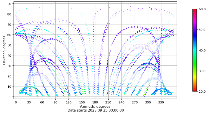
Azimuth-elevation plot for station RIO1. Signal to Noise S1C Data file RIO100ESP_R_2023268.xtr
