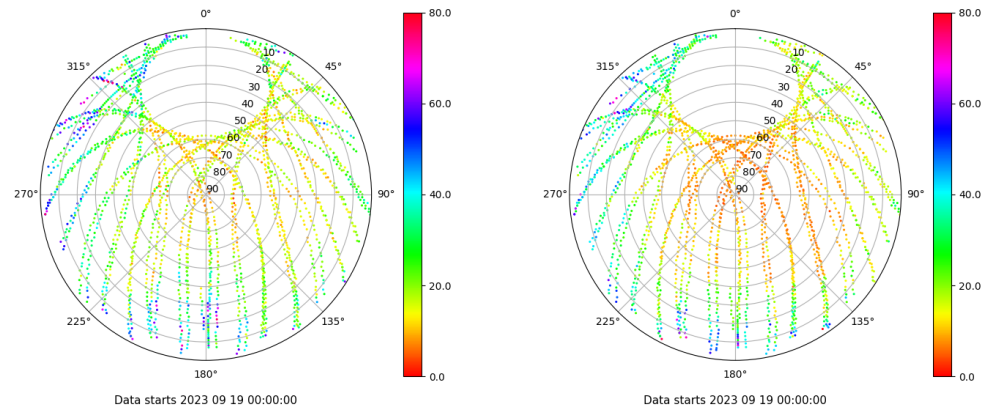
Skyplot for station RIO1. Parameter M1C Data file RIO100ESP_R_2023262.xtr Skyplot for station RIO1. Parameter M2P Data file RIO100ESP_R_2023262.xtr
