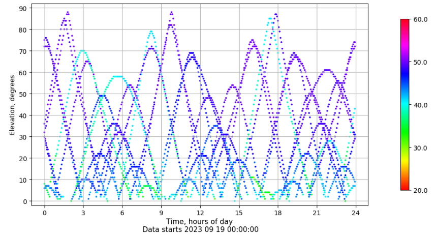
Time-elevation plot for station RIO1. Signal to Noise S1C Data file RIO100ESP_R_2023262.xtr
