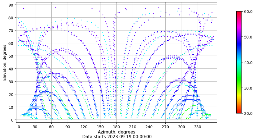
Azimuth-elevation plot for station RIO1. Signal to Noise S1C Data file RIO100ESP_R_2023262.xtr
