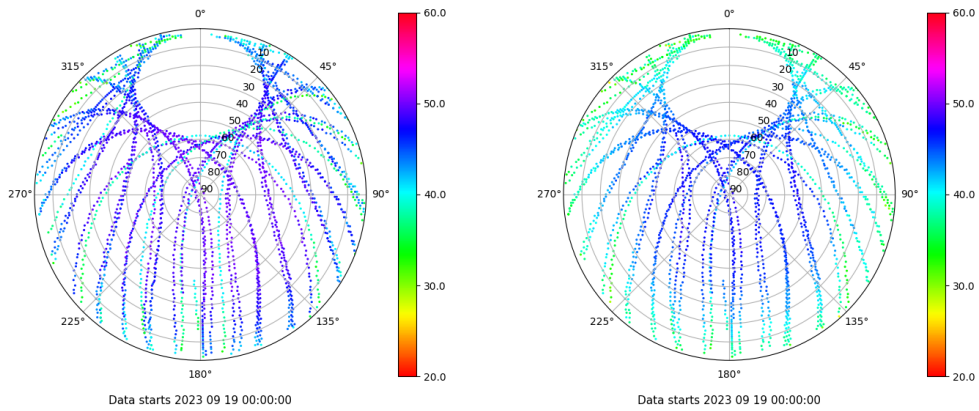
Skyplot for station RIO1. Signal to Noise S1C Data file RIO100ESP_R_2023262.xtr Skyplot for station RIO1. Signal to Noise S2P Data file RIO100ESP_R_2023262.xtr
