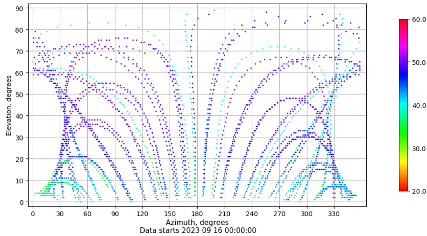
Azimuth-elevation plot for station RIO1. Signal to Noise S1C Data file RIO100ESP_R_2023259.xtr
