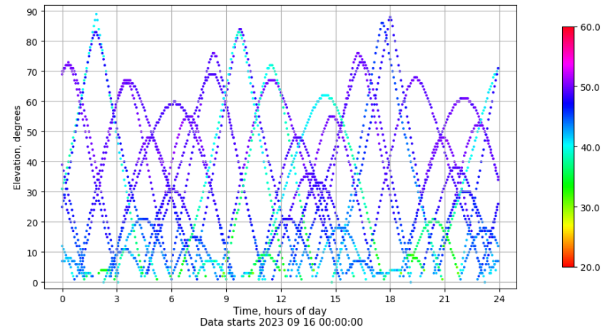
Time-elevation plot for station RIO1. Signal to Noise S1C Data file RIO100ESP_R_2023259.xtr
