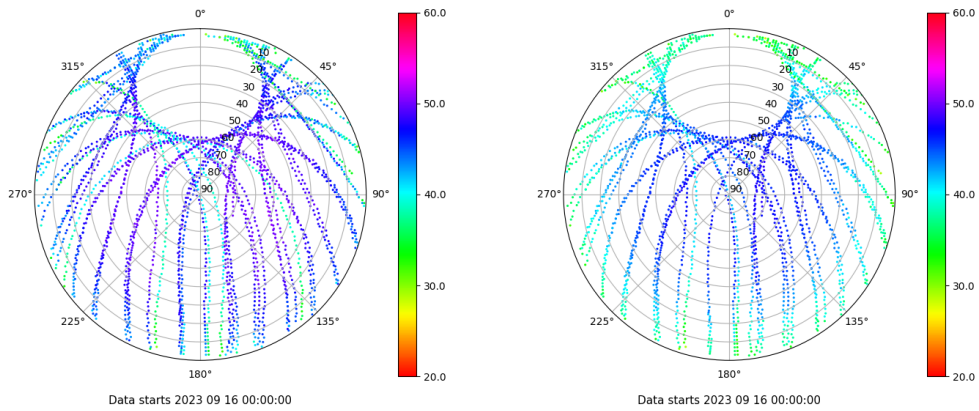
Skyplot for station RIO1. Signal to Noise S1C Data file RIO100ESP_R_2023259.xtr Skyplot for station RIO1. Signal to Noise S2P Data file RIO100ESP_R_2023259.xtr
