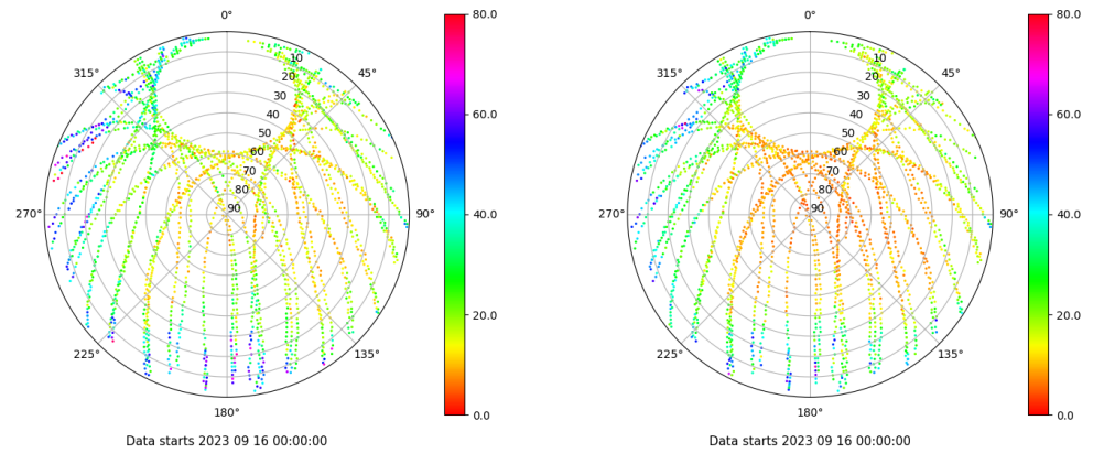
Skyplot for station RIO1. Parameter M1C Data file RIO100ESP_R_2023259.xtr Skyplot for station RIO1. Parameter M2P Data file RIO100ESP_R_2023259.xtr
