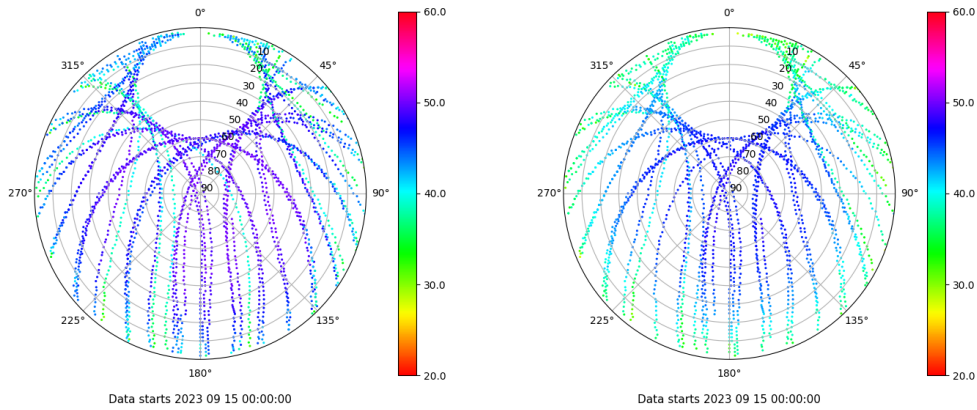
Skyplot for station RIO1. Signal to Noise S1C Data file RIO100ESP_R_2023258.xtr Skyplot for station RIO1. Signal to Noise S2P Data file RIO100ESP_R_2023258.xtr
