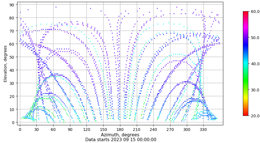
Azimuth-elevation plot for station RIO1. Signal to Noise S1C Data file RIO100ESP_R_2023258.xtr
