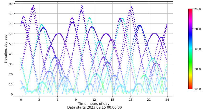
Time-elevation plot for station RIO1. Signal to Noise S1C Data file RIO100ESP_R_2023258.xtr
