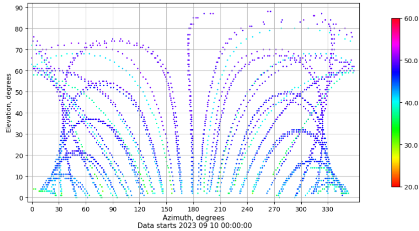
Azimuth-elevation plot for station RIO1. Signal to Noise S1C Data file RIO100ESP_R_2023253.xtr
