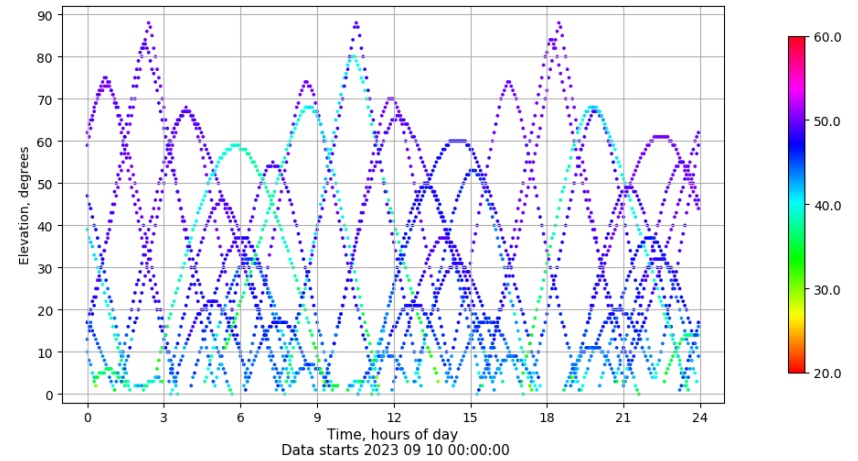
Time-elevation plot for station RIO1. Signal to Noise S1C Data file RIO100ESP_R_2023253.xtr
