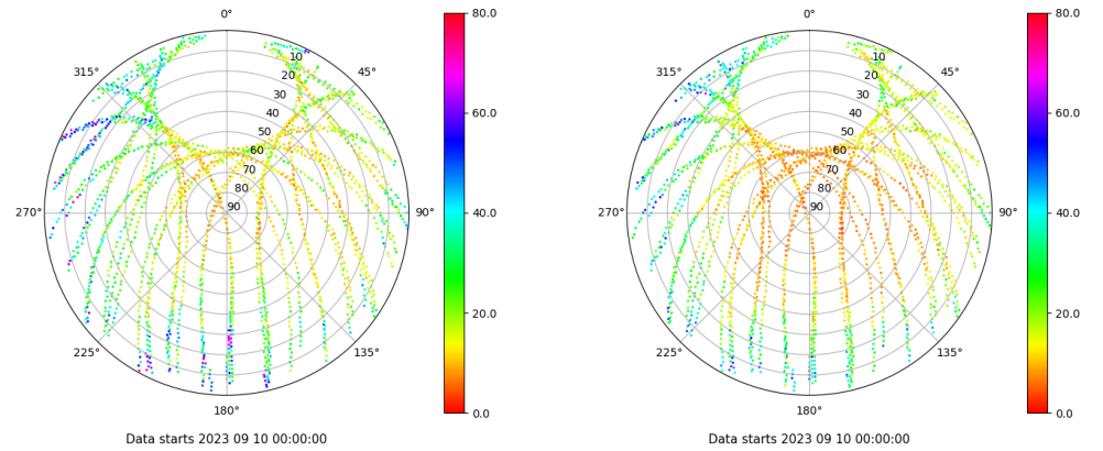
Skyplot for station RIO1. Parameter M1C Data file RIO100ESP_R_2023253.xtr Skyplot for station RIO1. Parameter M2P Data file RIO100ESP_R_2023253.xtr
