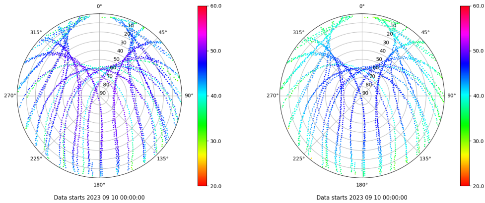
Skyplot for station RIO1. Signal to Noise S1C Data file RIO100ESP_R_2023253.xtr Skyplot for station RIO1. Signal to Noise S2P Data file RIO100ESP_R_2023253.xtr
