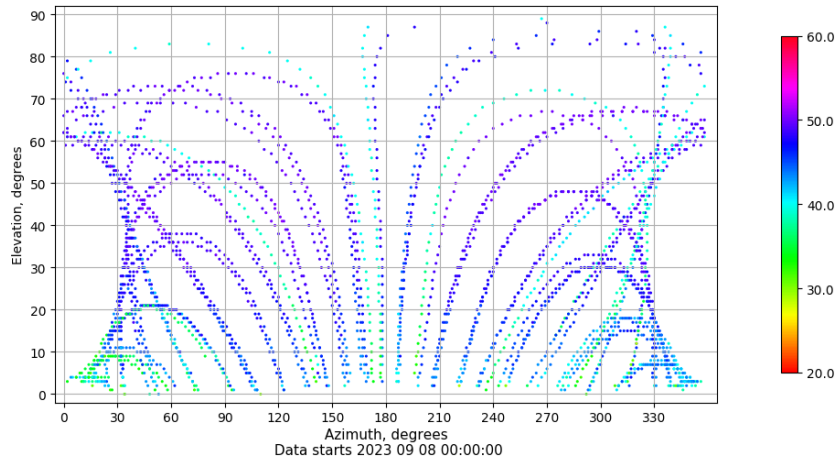
Azimuth-elevation plot for station RIO1. Signal to Noise S1C Data file RIO100ESP_R_2023251.xtr
