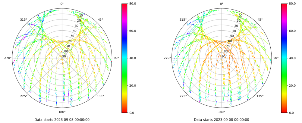
Skyplot for station RIO1. Parameter M1C Data file RIO100ESP_R_2023251.xtr Skyplot for station RIO1. Parameter M2P Data file RIO100ESP_R_2023251.xtr
