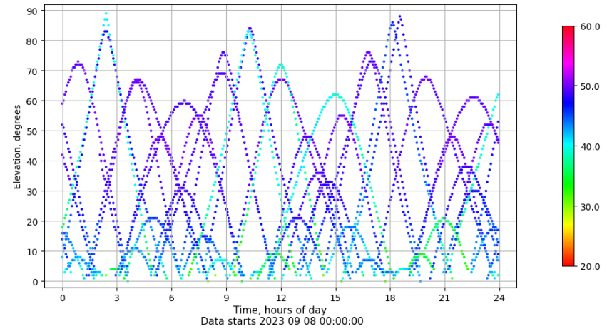
Time-elevation plot for station RIO1. Signal to Noise S1C Data file RIO100ESP_R_2023251.xtr
