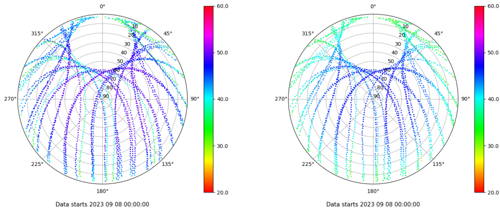
Skyplot for station RIO1. Signal to Noise S1C Data file RIO100ESP_R_2023251.xtr Skyplot for station RIO1. Signal to Noise S2P Data file RIO100ESP_R_2023251.xtr
