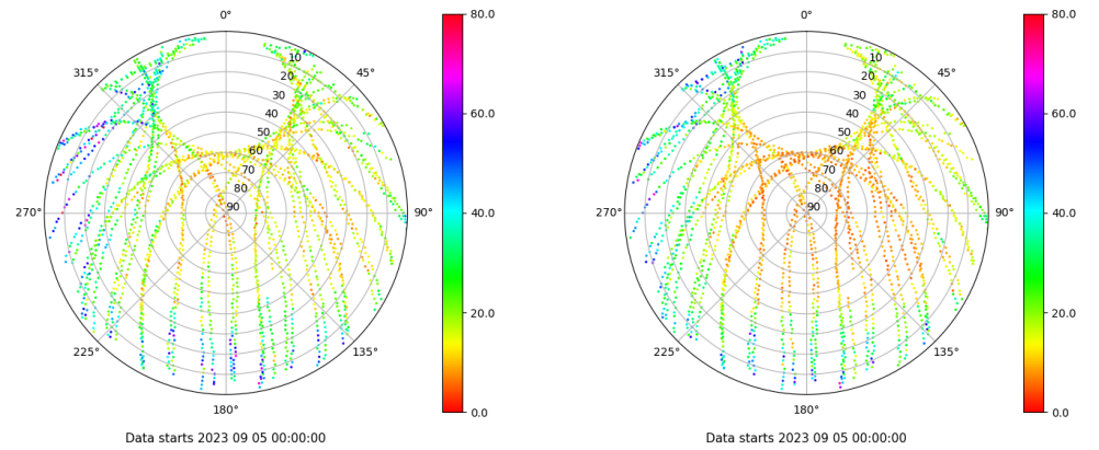
Skyplot for station RIO1. Parameter M1C Data file RIO100ESP_R_2023248.xtr Skyplot for station RIO1. Parameter M2P Data file RIO100ESP_R_2023248.xtr
