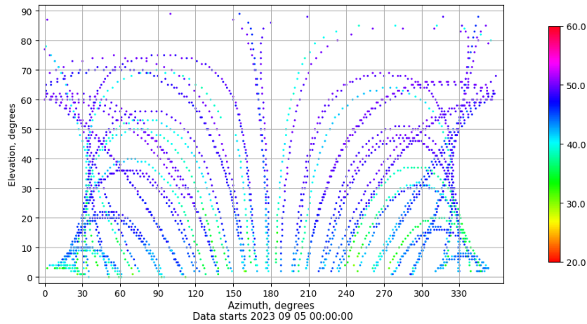
Azimuth-elevation plot for station RIO1. Signal to Noise S1C Data file RIO100ESP_R_2023248.xtr
