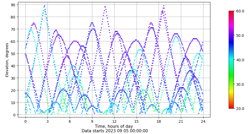
Time-elevation plot for station RIO1. Signal to Noise S1C Data file RIO100ESP_R_2023248.xtr
