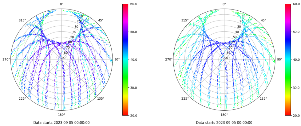
Skyplot for station RIO1. Signal to Noise S1C Data file RIO100ESP_R_2023248.xtr Skyplot for station RIO1. Signal to Noise S2P Data file RIO100ESP_R_2023248.xtr
