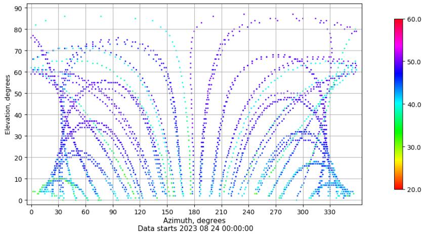
Azimuth-elevation plot for station RIO1. Signal to Noise S1C Data file RIO100ESP_R_2023236.xtr
