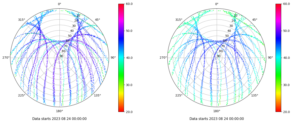
Skyplot for station RIO1. Signal to Noise S1C Data file RIO100ESP_R_2023236.xtr Skyplot for station RIO1. Signal to Noise S2P Data file RIO100ESP_R_2023236.xtr
