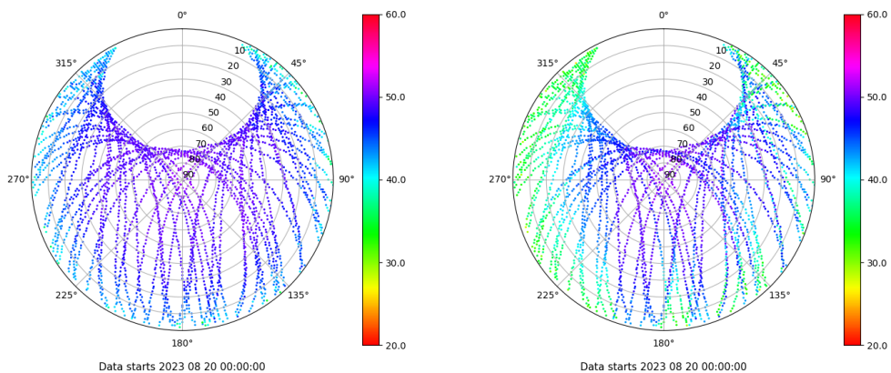
Skyplot for station RIO1. Signal to Noise S1C Data file RIO100ESP_R_2023232.xtr Skyplot for station RIO1. Signal to Noise S2W Data file RIO100ESP_R_2023232.xtr
