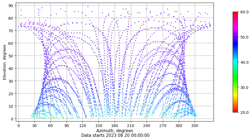
Azimuth-elevation plot for station RIO1. Signal to Noise S1C Data file RIO100ESP_R_2023232.xtr
