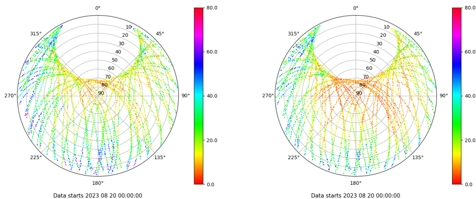
Skyplot for station RIO1. Parameter M1C Data file RIO100ESP_R_2023232.xtr Skyplot for station RIO1. Parameter M2W Data file RIO100ESP_R_2023232.xtr
