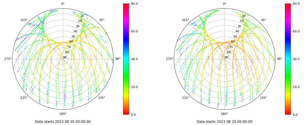
Skyplot for station RIO1. Parameter M1C Data file RIO100ESP_R_2023232.xtr Skyplot for station RIO1. Parameter M2P Data file RIO100ESP_R_2023232.xtr
