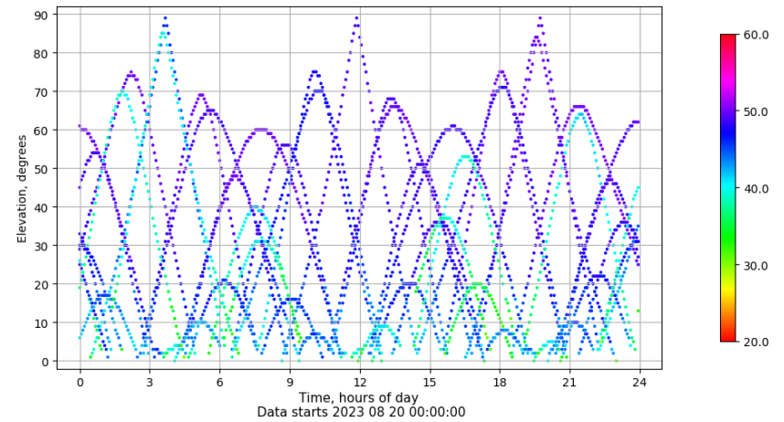
Time-elevation plot for station RIO1. Signal to Noise S1C Data file RIO100ESP_R_2023232.xtr
