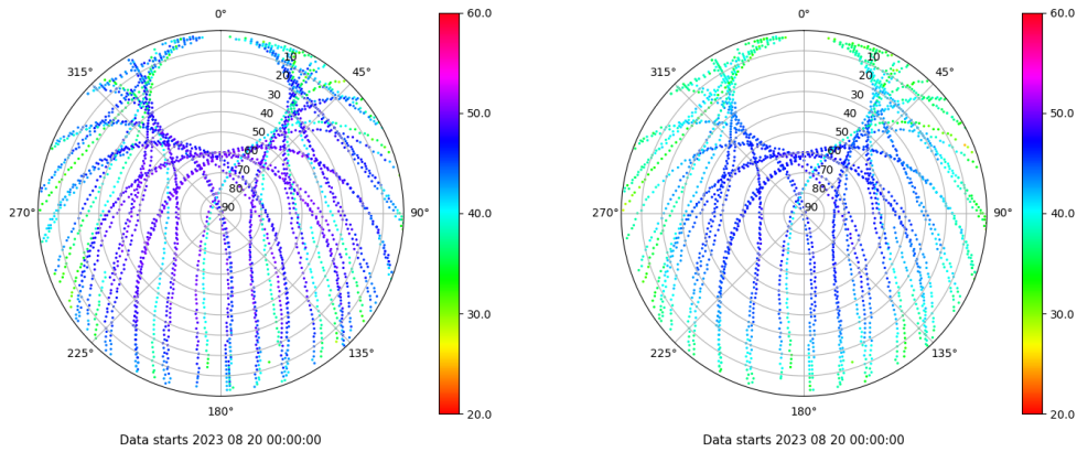
Skyplot for station RIO1. Signal to Noise S1C Data file RIO100ESP_R_2023232.xtr Skyplot for station RIO1. Signal to Noise S2P Data file RIO100ESP_R_2023232.xtr
