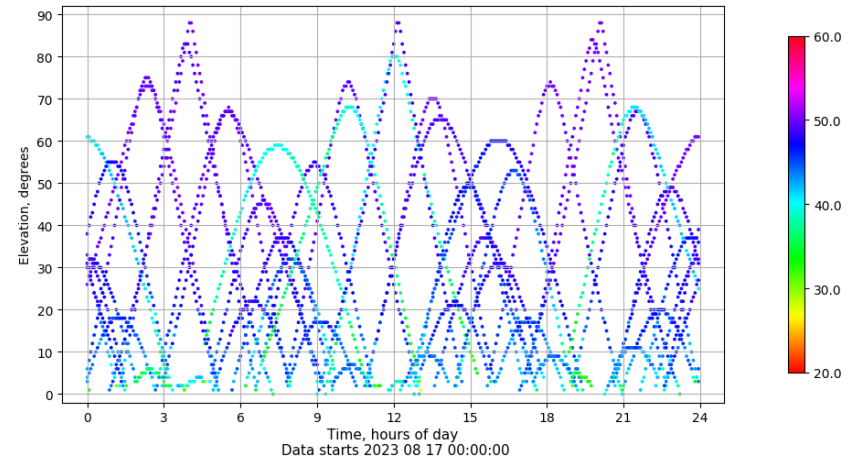
Time-elevation plot for station RIO1. Signal to Noise S1C Data file RIO100ESP_R_2023229.xtr
