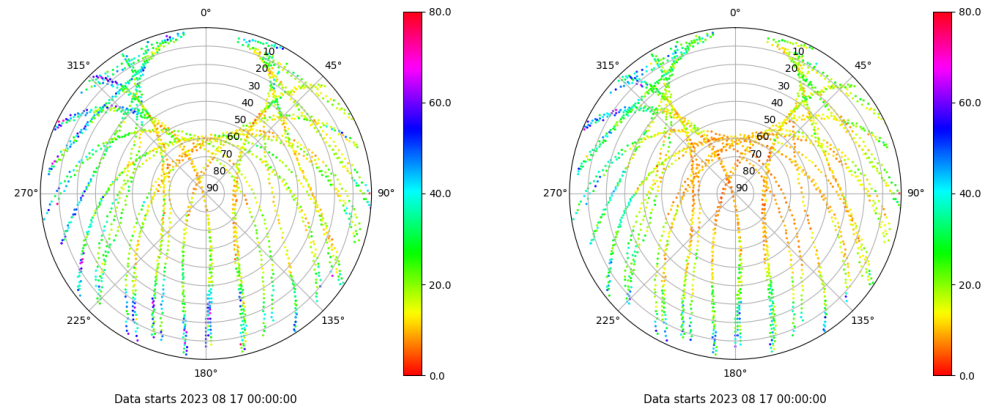
Skyplot for station RIO1. Parameter M1C Data file RIO100ESP_R_2023229.xtr Skyplot for station RIO1. Parameter M2P Data file RIO100ESP_R_2023229.xtr
