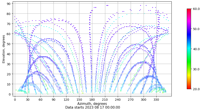
Azimuth-elevation plot for station RIO1. Signal to Noise S1C Data file RIO100ESP_R_2023229.xtr
