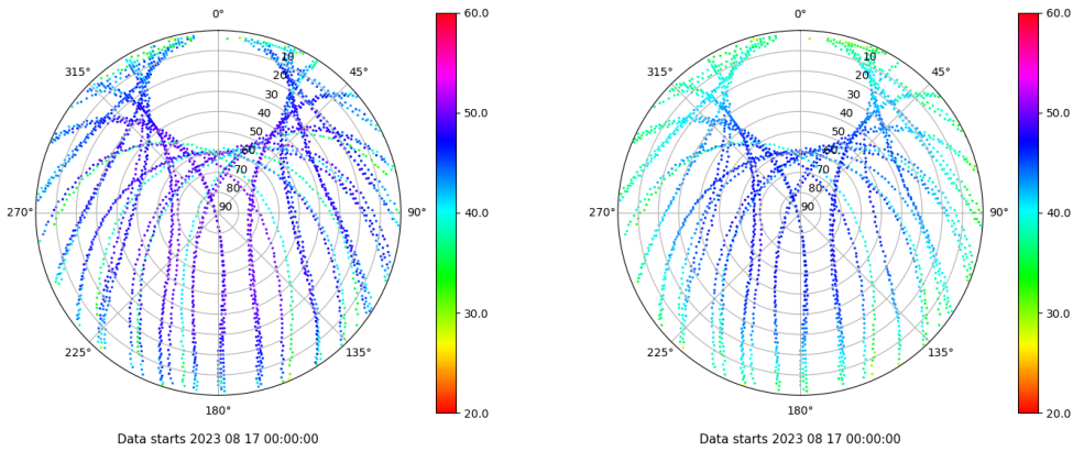
Skyplot for station RIO1. Signal to Noise S1C Data file RIO100ESP_R_2023229.xtr Skyplot for station RIO1. Signal to Noise S2P Data file RIO100ESP_R_2023229.xtr
