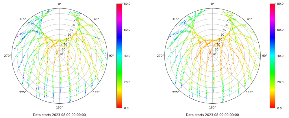
Skyplot for station RIO1. Parameter M1C Data file RIO100ESP_R_2023221.xtr Skyplot for station RIO1. Parameter M2P Data file RIO100ESP_R_2023221.xtr
