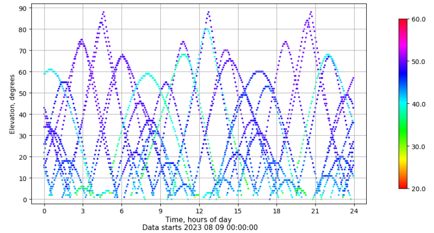
Time-elevation plot for station RIO1. Signal to Noise S1C Data file RIO100ESP_R_2023221.xtr
