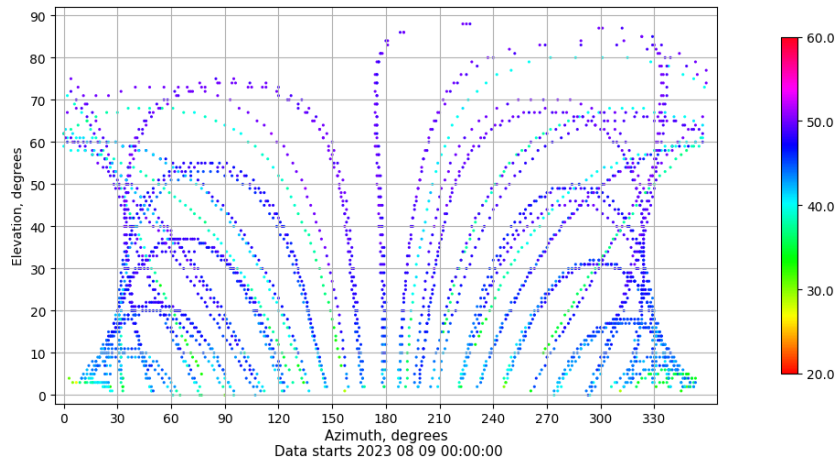
Azimuth-elevation plot for station RIO1. Signal to Noise S1C Data file RIO100ESP_R_2023221.xtr
