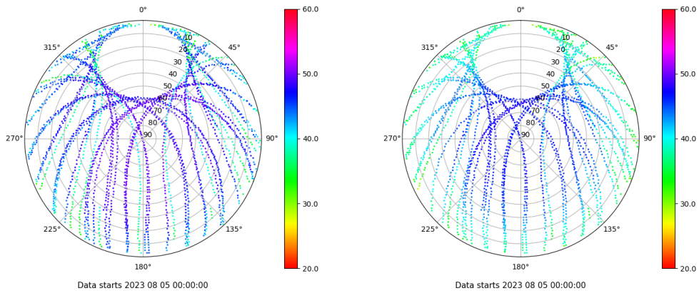
Skyplot for station RIO1. Signal to Noise S1C Data file RIO100ESP_R_2023217.xtr Skyplot for station RIO1. Signal to Noise S2P Data file RIO100ESP_R_2023217.xtr
