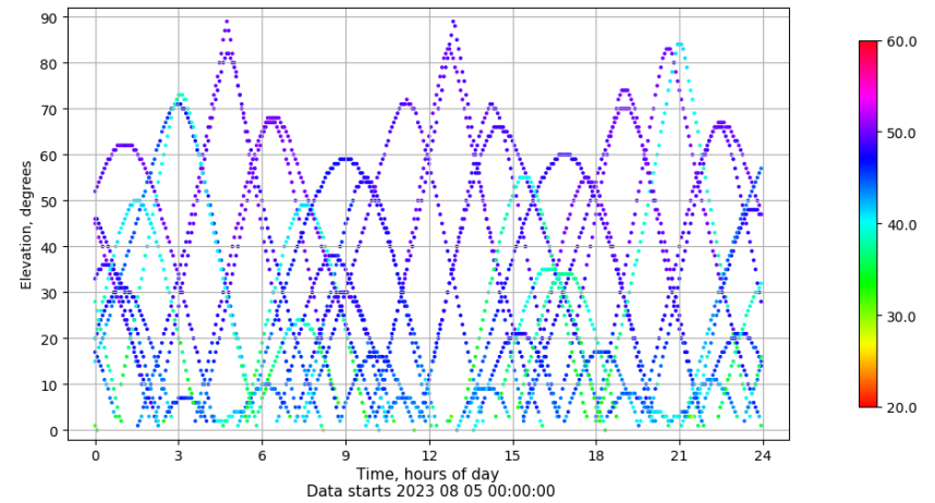
Time-elevation plot for station RIO1. Signal to Noise S1C Data file RIO100ESP_R_2023217.xtr
