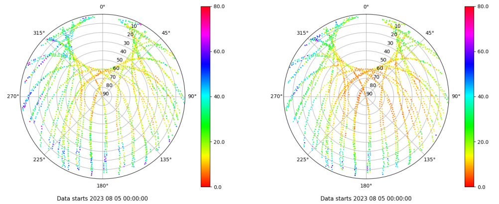
Skyplot for station RIO1. Parameter M1C Data file RIO100ESP_R_2023217.xtr Skyplot for station RIO1. Parameter M2P Data file RIO100ESP_R_2023217.xtr
