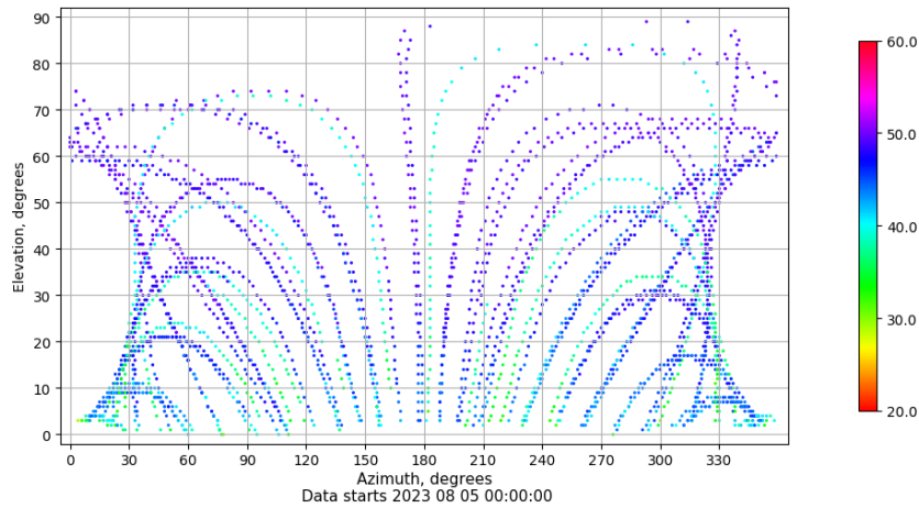
Azimuth-elevation plot for station RIO1. Signal to Noise S1C Data file RIO100ESP_R_2023217.xtr
