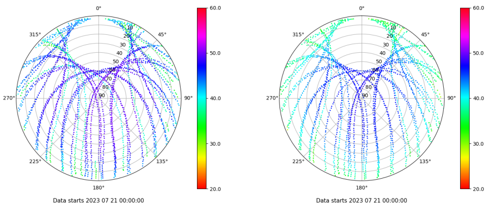
Skyplot for station RIO1. Signal to Noise S1C Data file RIO100ESP_R_2023202.xtr Skyplot for station RIO1. Signal to Noise S2P Data file RIO100ESP_R_2023202.xtr
