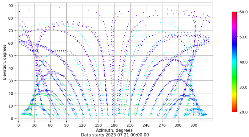
Azimuth-elevation plot for station RIO1. Signal to Noise S1C Data file RIO100ESP_R_2023202.xtr
