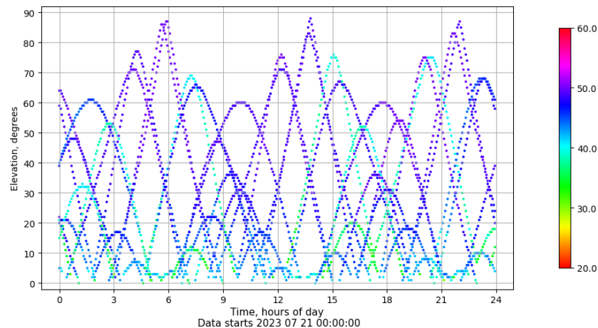
Time-elevation plot for station RIO1. Signal to Noise S1C Data file RIO100ESP_R_2023202.xtr
