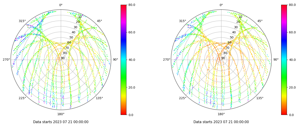
Skyplot for station RIO1. Parameter M1C Data file RIO100ESP_R_2023202.xtr Skyplot for station RIO1. Parameter M2P Data file RIO100ESP_R_2023202.xtr
