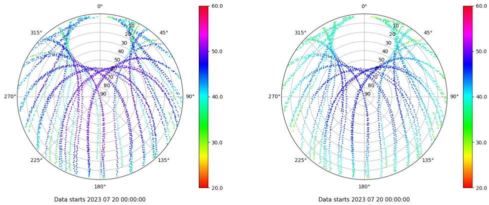
Skyplot for station RIO1. Signal to Noise S1C Data file RIO100ESP_R_2023201.xtr Skyplot for station RIO1. Signal to Noise S2P Data file RIO100ESP_R_2023201.xtr
