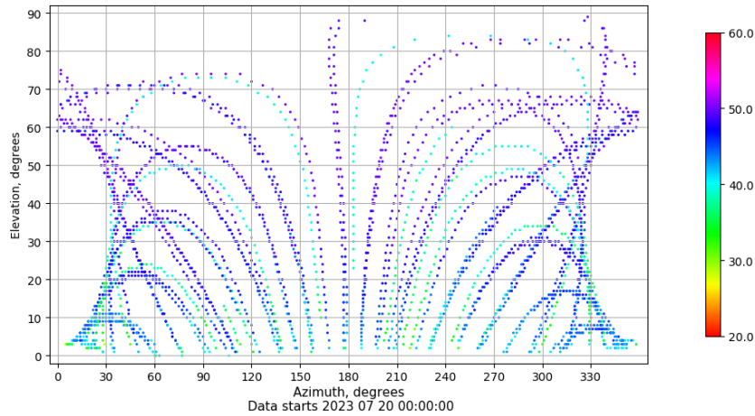
Azimuth-elevation plot for station RIO1. Signal to Noise S1C Data file RIO100ESP_R_2023201.xtr
