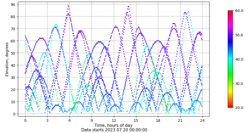
Time-elevation plot for station RIO1. Signal to Noise S1C Data file RIO100ESP_R_2023201.xtr
