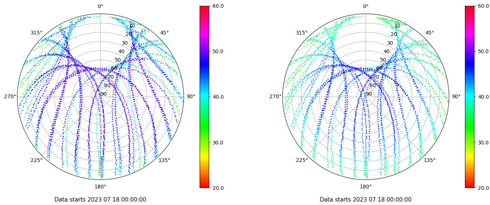
Skyplot for station RIO1. Signal to Noise S1C Data file RIO100ESP_R_2023199.xtr Skyplot for station RIO1. Signal to Noise S2P Data file RIO100ESP_R_2023199.xtr
