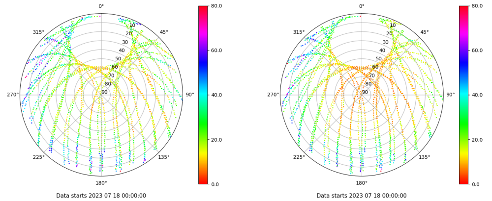
Skyplot for station RIO1. Parameter M1C Data file RIO100ESP_R_2023199.xtr Skyplot for station RIO1. Parameter M2P Data file RIO100ESP_R_2023199.xtr
