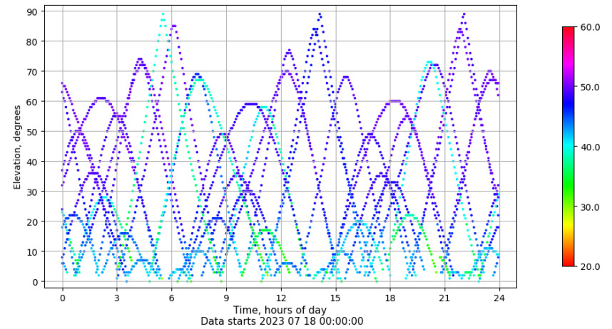
Time-elevation plot for station RIO1. Signal to Noise S1C Data file RIO100ESP_R_2023199.xtr
