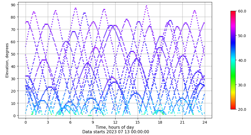
Time-elevation plot for station RIO1. Signal to Noise S1C Data file RIO100ESP_R_2023194.xtr
