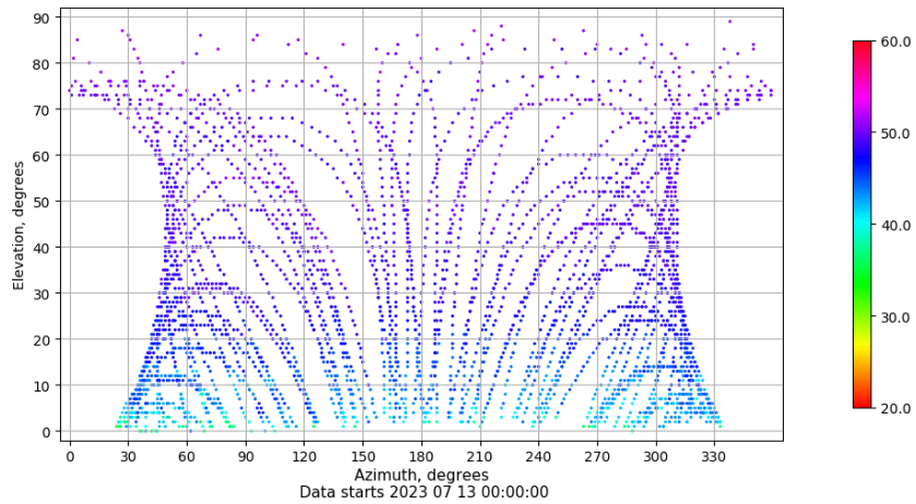
Azimuth-elevation plot for station RIO1. Signal to Noise S1C Data file RIO100ESP_R_2023194.xtr
