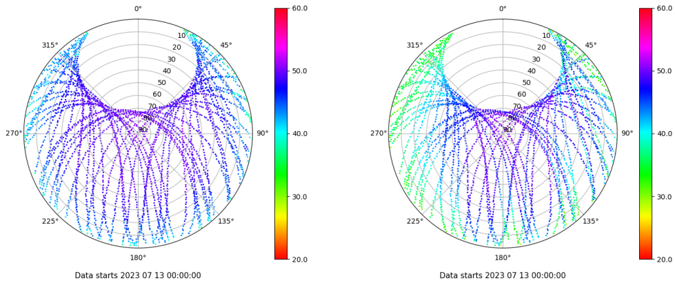
Skyplot for station RIO1. Signal to Noise S1C Data file RIO100ESP_R_2023194.xtr Skyplot for station RIO1. Signal to Noise S2W Data file RIO100ESP_R_2023194.xtr
