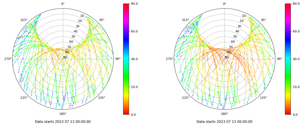
Skyplot for station RIO1. Parameter M1C Data file RIO100ESP_R_2023194.xtr Skyplot for station RIO1. Parameter M2W Data file RIO100ESP_R_2023194.xtr
