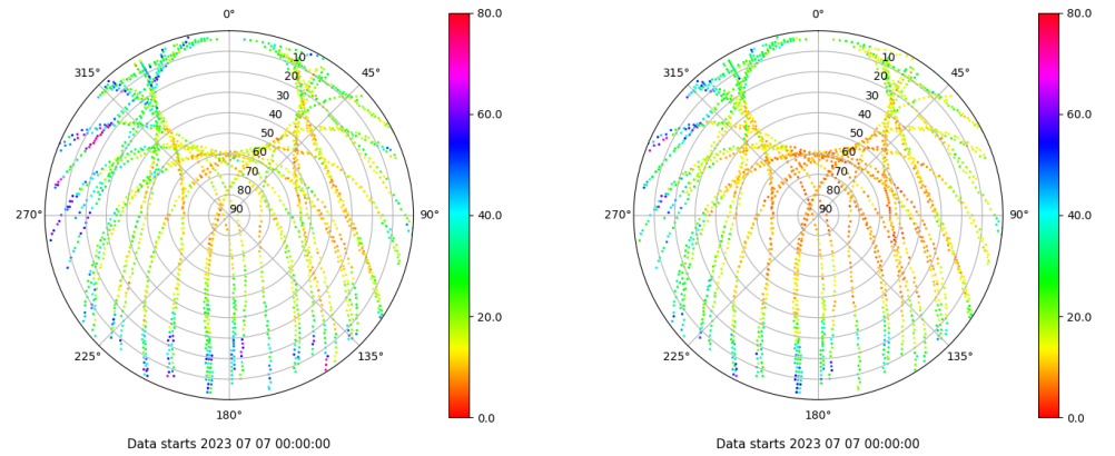
Skyplot for station RIO1. Parameter M1C Data file RIO100ESP_R_2023188.xtr Skyplot for station RIO1. Parameter M2P Data file RIO100ESP_R_2023188.xtr
