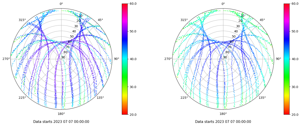
Skyplot for station RIO1. Signal to Noise S1C Data file RIO100ESP_R_2023188.xtr Skyplot for station RIO1. Signal to Noise S2P Data file RIO100ESP_R_2023188.xtr
