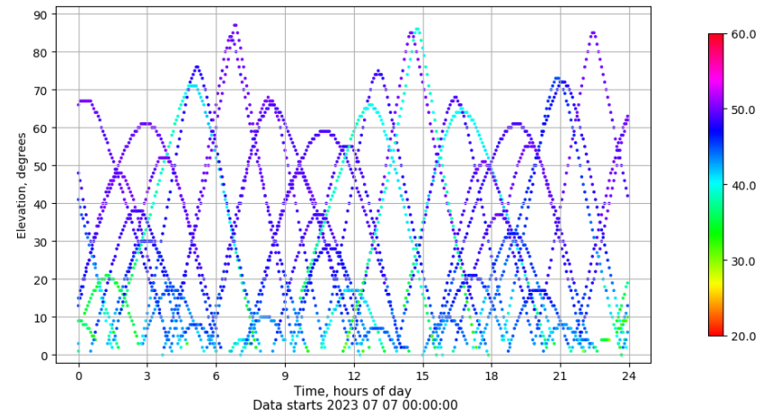
Time-elevation plot for station RIO1. Signal to Noise S1C Data file RIO100ESP_R_2023188.xtr
