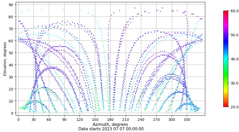
Azimuth-elevation plot for station RIO1. Signal to Noise S1C Data file RIO100ESP_R_2023188.xtr
