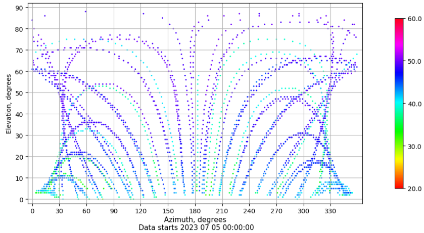
Azimuth-elevation plot for station RIO1. Signal to Noise S1C Data file RIO100ESP_R_2023186.xtr
