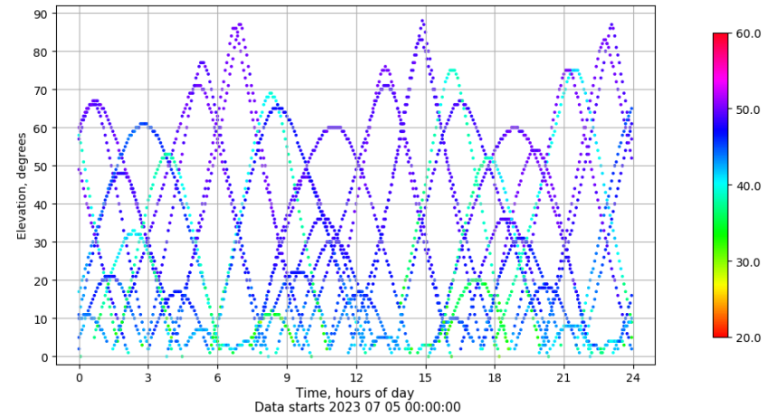
Time-elevation plot for station RIO1. Signal to Noise S1C Data file RIO100ESP_R_2023186.xtr
