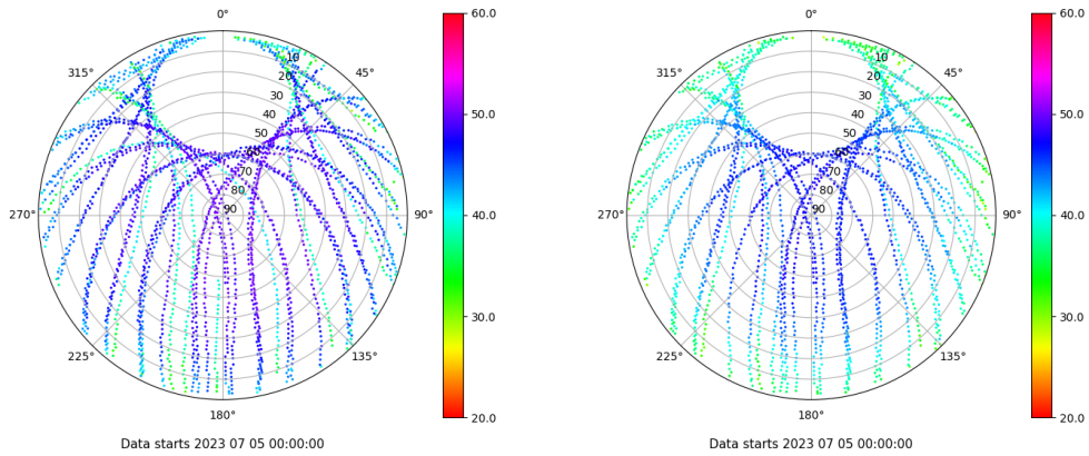
Skyplot for station RIO1. Signal to Noise S1C Data file RIO100ESP_R_2023186.xtr Skyplot for station RIO1. Signal to Noise S2P Data file RIO100ESP_R_2023186.xtr
