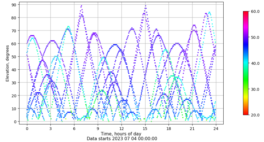
Time-elevation plot for station RIO1. Signal to Noise S1C Data file RIO100ESP_R_2023185.xtr
