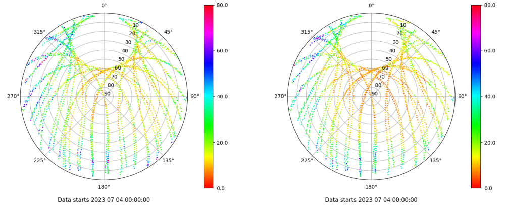
Skyplot for station RIO1. Parameter M1C Data file RIO100ESP_R_2023185.xtr Skyplot for station RIO1. Parameter M2P Data file RIO100ESP_R_2023185.xtr
