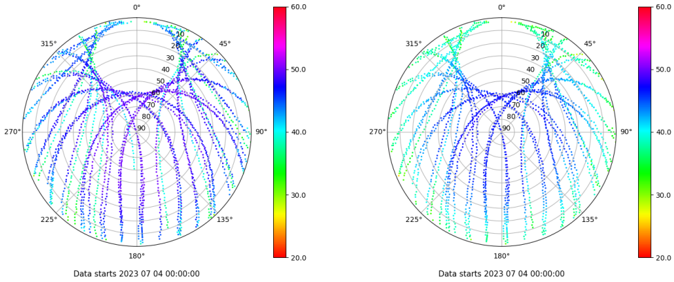
Skyplot for station RIO1. Signal to Noise S1C Data file RIO100ESP_R_2023185.xtr Skyplot for station RIO1. Signal to Noise S2P Data file RIO100ESP_R_2023185.xtr
