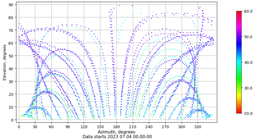
Azimuth-elevation plot for station RIO1. Signal to Noise S1C Data file RIO100ESP_R_2023185.xtr
