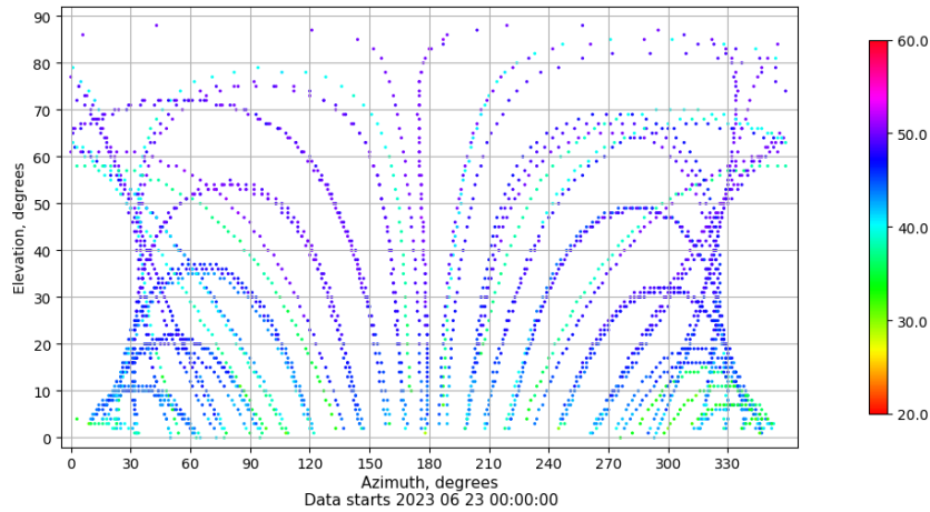
Azimuth-elevation plot for station RIO1. Signal to Noise S1C Data file RIO100ESP_R_2023174.xtr
