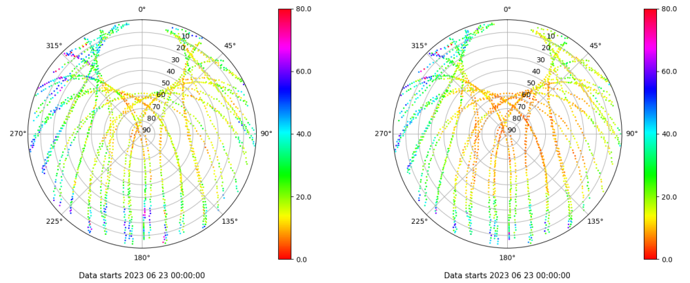
Skyplot for station RIO1. Parameter M1C Data file RIO100ESP_R_2023174.xtr Skyplot for station RIO1. Parameter M2P Data file RIO100ESP_R_2023174.xtr
