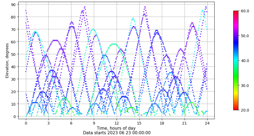
Time-elevation plot for station RIO1. Signal to Noise S1C Data file RIO100ESP_R_2023174.xtr
