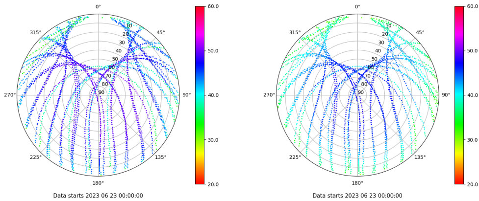
Skyplot for station RIO1. Signal to Noise S1C Data file RIO100ESP_R_2023174.xtr Skyplot for station RIO1. Signal to Noise S2P Data file RIO100ESP_R_2023174.xtr
