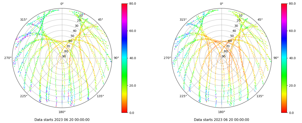
Skyplot for station RIO1. Parameter M1C Data file RIO100ESP_R_2023171.xtr Skyplot for station RIO1. Parameter M2P Data file RIO100ESP_R_2023171.xtr
