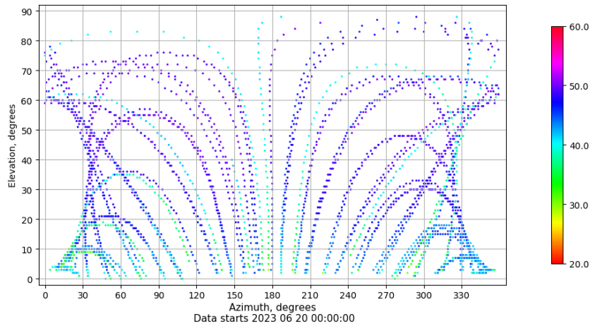
Azimuth-elevation plot for station RIO1. Signal to Noise S1C Data file RIO100ESP_R_2023171.xtr
