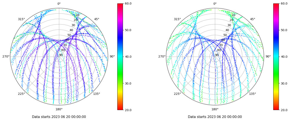
Skyplot for station RIO1. Signal to Noise S1C Data file RIO100ESP_R_2023171.xtr Skyplot for station RIO1. Signal to Noise S2P Data file RIO100ESP_R_2023171.xtr
