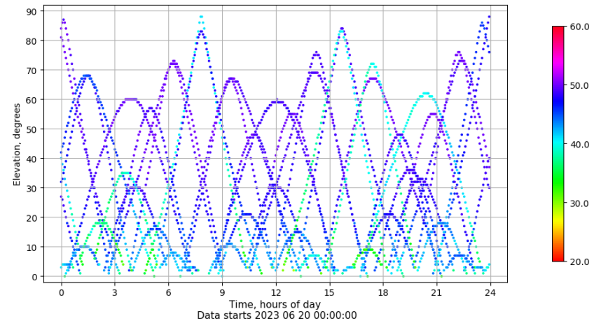
Time-elevation plot for station RIO1. Signal to Noise S1C Data file RIO100ESP_R_2023171.xtr
