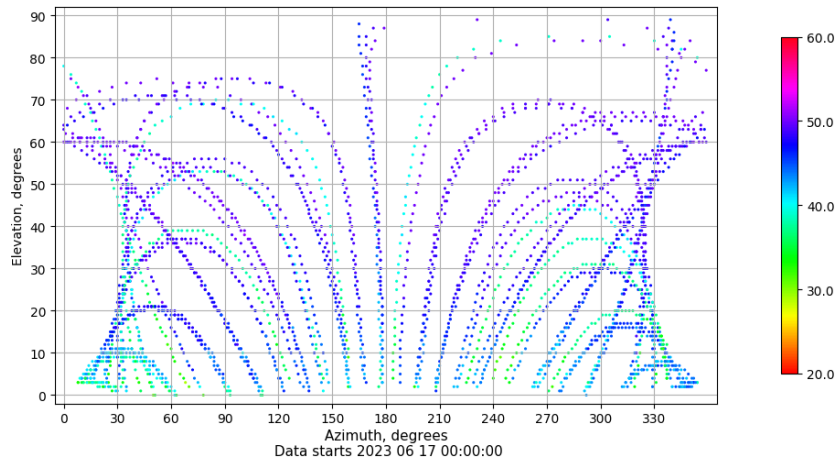
Azimuth-elevation plot for station RIO1. Signal to Noise S1C Data file RIO100ESP_R_2023168.xtr
