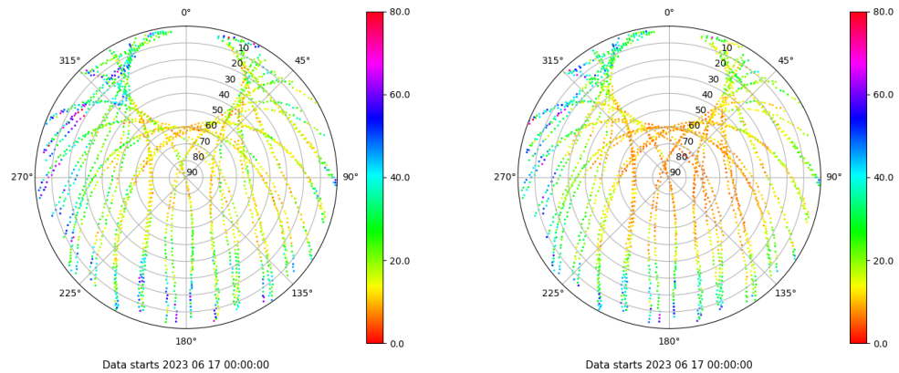
Skyplot for station RIO1. Parameter M1C Data file RIO100ESP_R_2023168.xtr Skyplot for station RIO1. Parameter M2P Data file RIO100ESP_R_2023168.xtr
