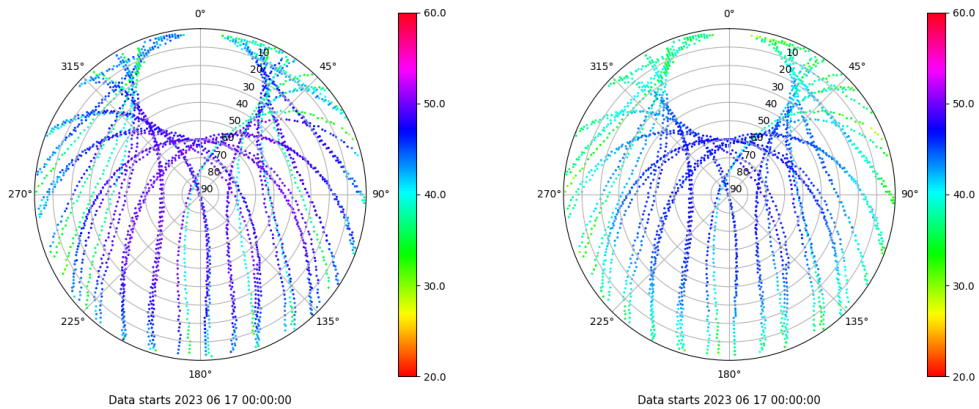
Skyplot for station RIO1. Signal to Noise S1C Data file RIO100ESP_R_2023168.xtr Skyplot for station RIO1. Signal to Noise S2P Data file RIO100ESP_R_2023168.xtr
