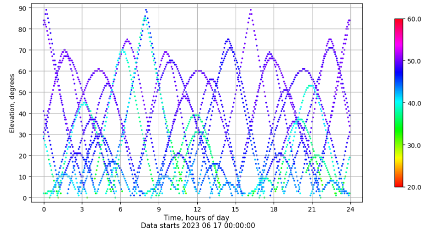
Time-elevation plot for station RIO1. Signal to Noise S1C Data file RIO100ESP_R_2023168.xtr
