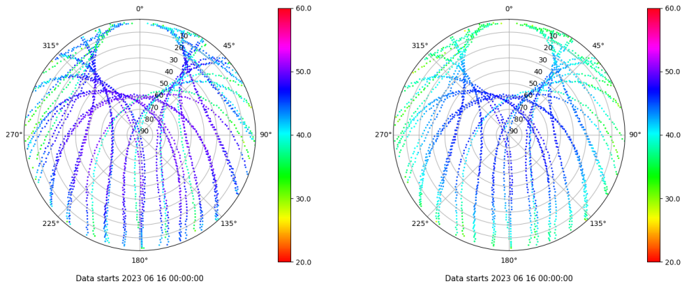
Skyplot for station RIO1. Signal to Noise S1C Data file RIO100ESP_R_2023167.xtr Skyplot for station RIO1. Signal to Noise S2P Data file RIO100ESP_R_2023167.xtr
