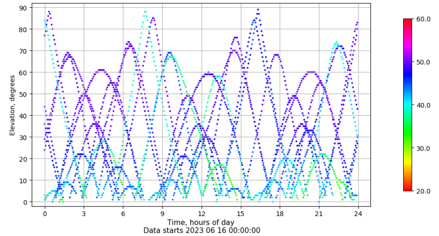
Time-elevation plot for station RIO1. Signal to Noise S1C Data file RIO100ESP_R_2023167.xtr
