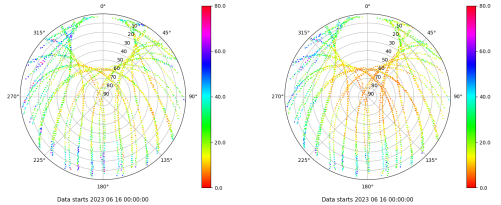
Skyplot for station RIO1. Parameter M1C Data file RIO100ESP_R_2023167.xtr Skyplot for station RIO1. Parameter M2P Data file RIO100ESP_R_2023167.xtr
