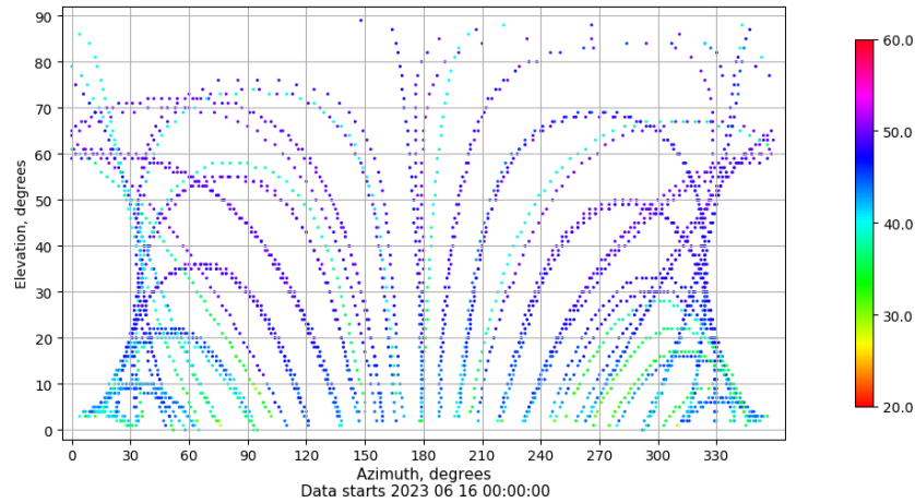
Azimuth-elevation plot for station RIO1. Signal to Noise S1C Data file RIO100ESP_R_2023167.xtr
