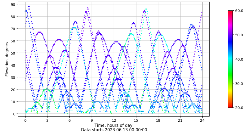
Time-elevation plot for station RIO1. Signal to Noise S1C Data file RIO100ESP_R_2023164.xtr
