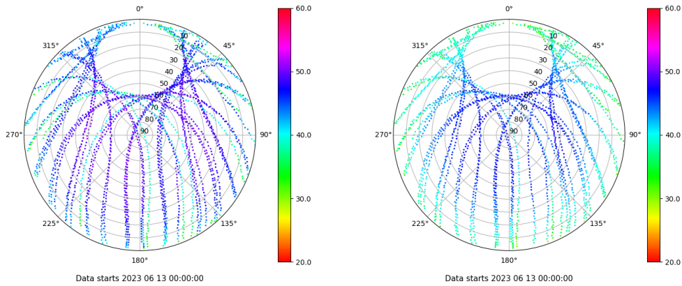
Skyplot for station RIO1. Signal to Noise S1C Data file RIO100ESP_R_2023164.xtr Skyplot for station RIO1. Signal to Noise S2P Data file RIO100ESP_R_2023164.xtr
