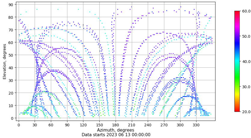
Azimuth-elevation plot for station RIO1. Signal to Noise S1C Data file RIO100ESP_R_2023164.xtr
