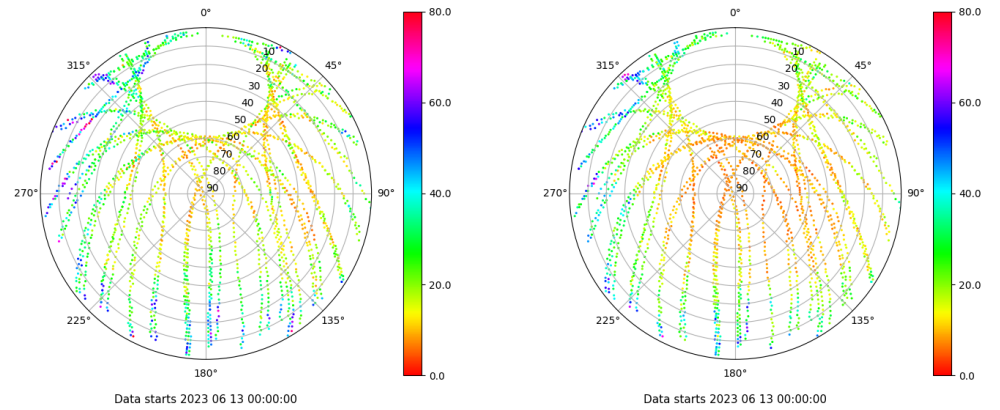
Skyplot for station RIO1. Parameter M1C Data file RIO100ESP_R_2023164.xtr Skyplot for station RIO1. Parameter M2P Data file RIO100ESP_R_2023164.xtr
