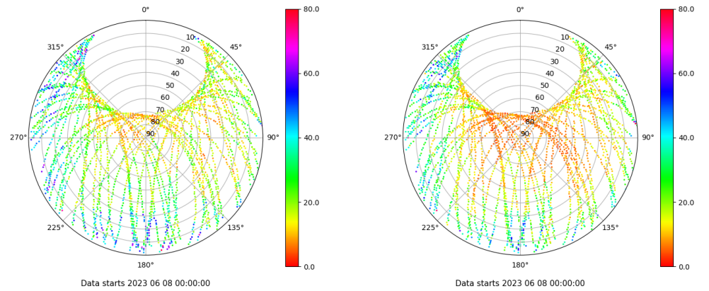
Skyplot for station RIO1. Parameter M1C Data file RIO100ESP_R_2023159.xtr Skyplot for station RIO1. Parameter M2W Data file RIO100ESP_R_2023159.xtr
