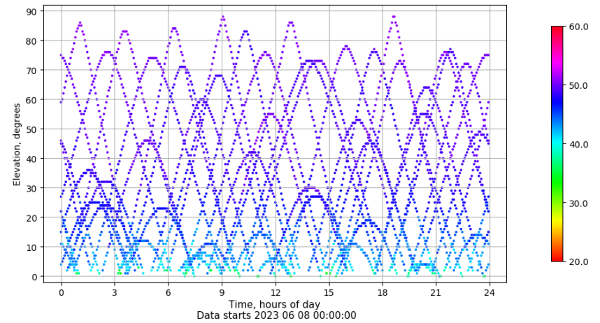
Time-elevation plot for station RIO1. Signal to Noise S1C Data file RIO100ESP_R_2023159.xtr
