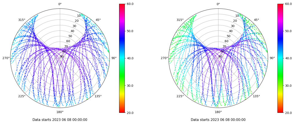
Skyplot for station RIO1. Signal to Noise S1C Data file RIO100ESP_R_2023159.xtr Skyplot for station RIO1. Signal to Noise S2W Data file RIO100ESP_R_2023159.xtr
