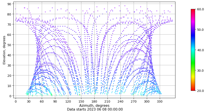
Azimuth-elevation plot for station RIO1. Signal to Noise S1C Data file RIO100ESP_R_2023159.xtr
