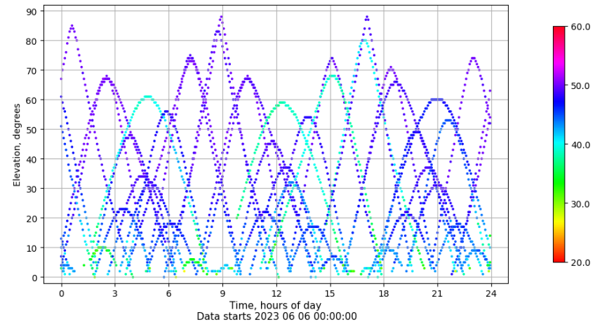
Time-elevation plot for station RIO1. Signal to Noise S1C Data file RIO100ESP_R_2023157.xtr
