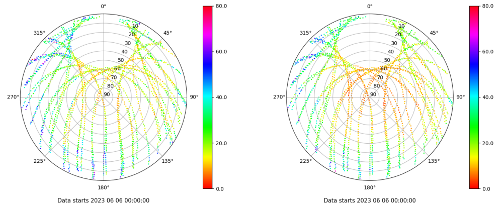
Skyplot for station RIO1. Parameter M1C Data file RIO100ESP_R_2023157.xtr Skyplot for station RIO1. Parameter M2P Data file RIO100ESP_R_2023157.xtr
