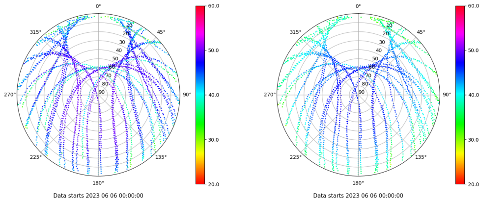
Skyplot for station RIO1. Signal to Noise S1C Data file RIO100ESP_R_2023157.xtr Skyplot for station RIO1. Signal to Noise S2P Data file RIO100ESP_R_2023157.xtr
