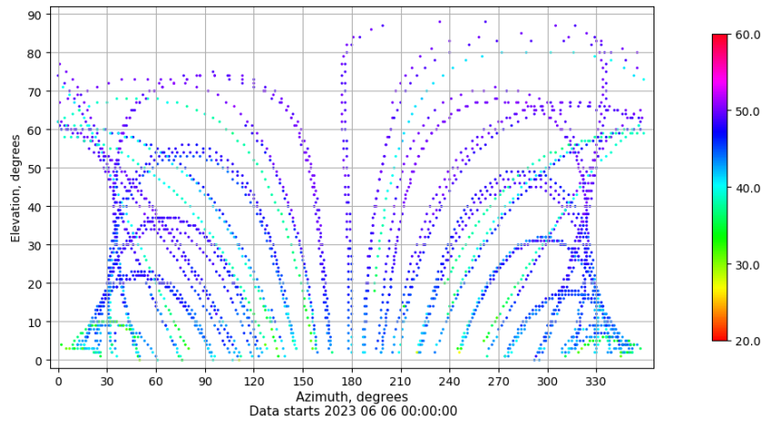
Azimuth-elevation plot for station RIO1. Signal to Noise S1C Data file RIO100ESP_R_2023157.xtr
