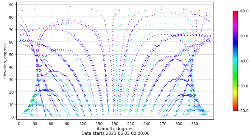
Azimuth-elevation plot for station RIO1. Signal to Noise S1C Data file RIO100ESP_R_2023154.xtr
