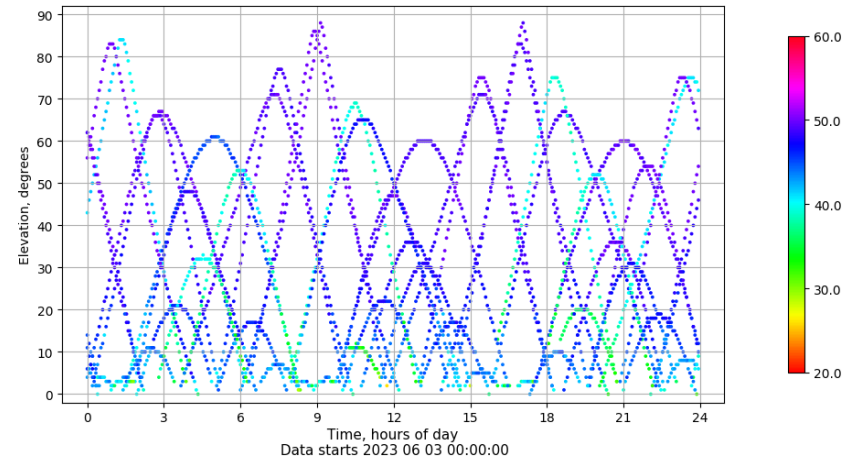
Time-elevation plot for station RIO1. Signal to Noise S1C Data file RIO100ESP_R_2023154.xtr
