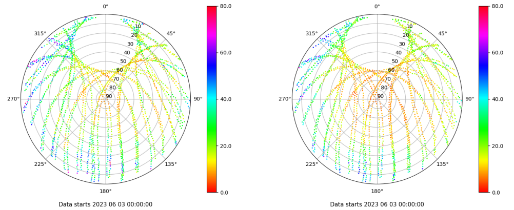
Skyplot for station RIO1. Parameter M1C Data file RIO100ESP_R_2023154.xtr Skyplot for station RIO1. Parameter M2P Data file RIO100ESP_R_2023154.xtr
