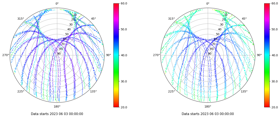
Skyplot for station RIO1. Signal to Noise S1C Data file RIO100ESP_R_2023154.xtr Skyplot for station RIO1. Signal to Noise S2P Data file RIO100ESP_R_2023154.xtr
