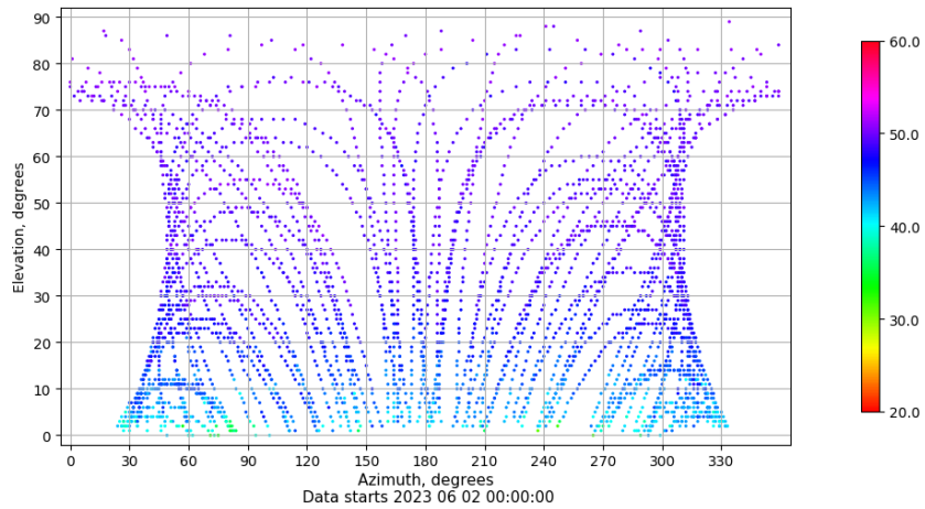
Azimuth-elevation plot for station RIO1. Signal to Noise S1C Data file RIO100ESP_R_2023153.xtr
