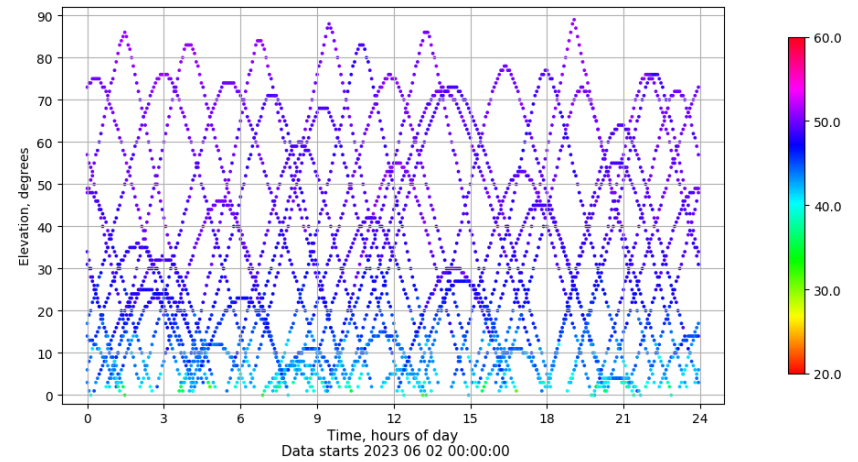
Time-elevation plot for station RIO1. Signal to Noise S1C Data file RIO100ESP_R_2023153.xtr
