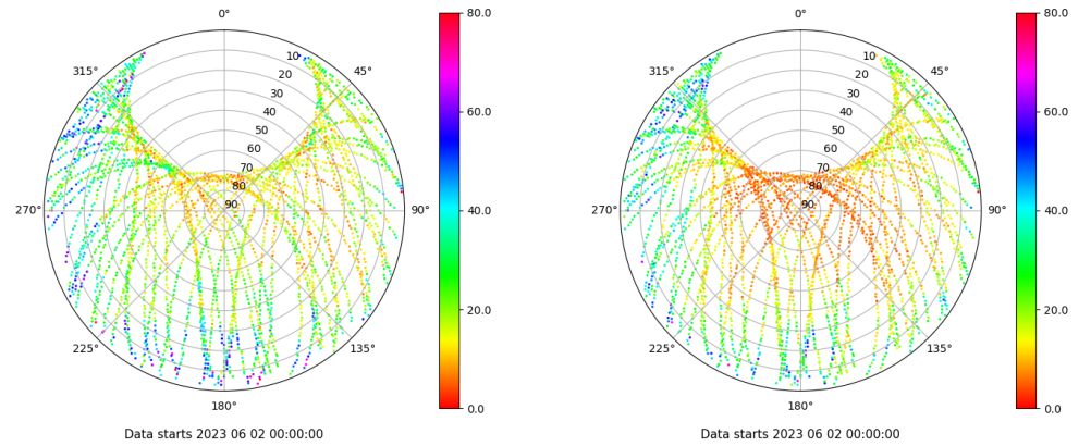
Skyplot for station RIO1. Parameter M1C Data file RIO100ESP_R_2023153.xtr Skyplot for station RIO1. Parameter M2W Data file RIO100ESP_R_2023153.xtr
