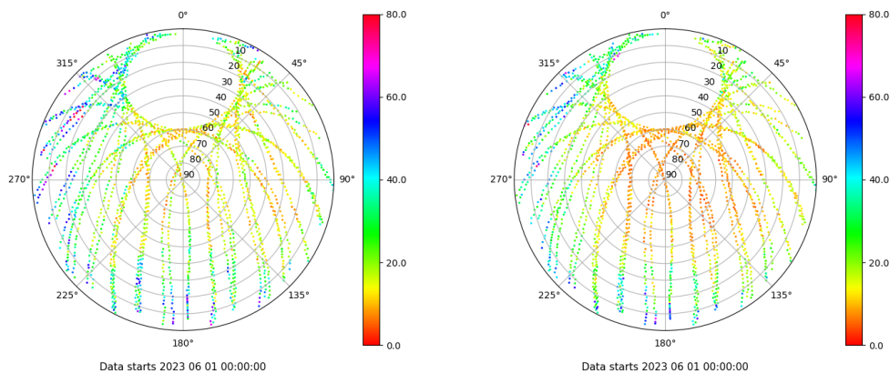
Skyplot for station RIO1. Parameter M1C Data file RIO100ESP_R_2023152.xtr Skyplot for station RIO1. Parameter M2P Data file RIO100ESP_R_2023152.xtr
