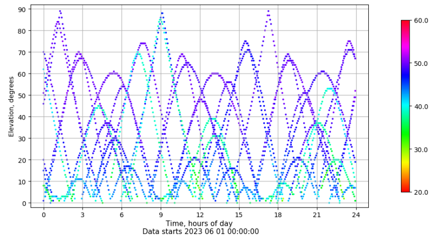
Time-elevation plot for station RIO1. Signal to Noise S1C Data file RIO100ESP_R_2023152.xtr
