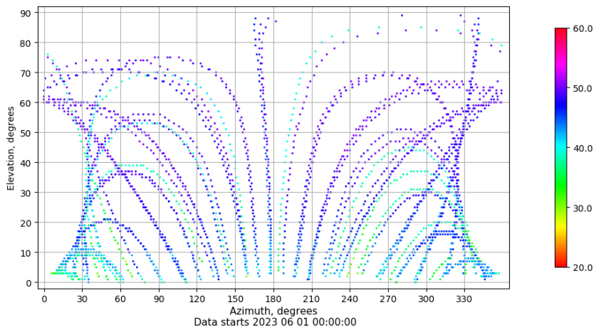
Azimuth-elevation plot for station RIO1. Signal to Noise S1C Data file RIO100ESP_R_2023152.xtr
