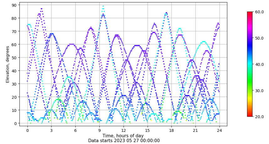
Time-elevation plot for station RIO1. Signal to Noise S1C Data file RIO100ESP_R_2023147.xtr
