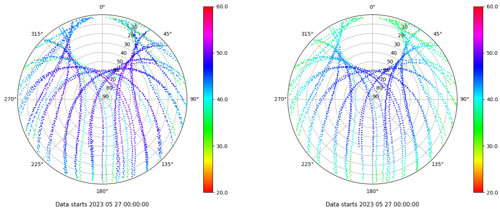
Skyplot for station RIO1. Signal to Noise S1C Data file RIO100ESP_R_2023147.xtr Skyplot for station RIO1. Signal to Noise S2P Data file RIO100ESP_R_2023147.xtr
