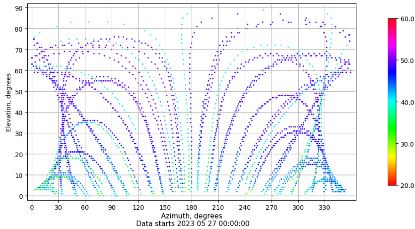
Azimuth-elevation plot for station RIO1. Signal to Noise S1C Data file RIO100ESP_R_2023147.xtr
