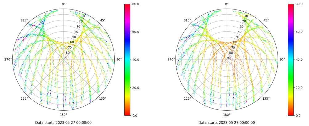
Skyplot for station RIO1. Parameter M1C Data file RIO100ESP_R_2023147.xtr Skyplot for station RIO1. Parameter M2P Data file RIO100ESP_R_2023147.xtr
