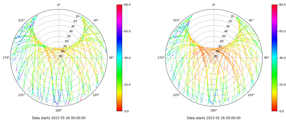
Skyplot for station RIO1. Parameter M1C Data file RIO100ESP_R_2023146.xtr Skyplot for station RIO1. Parameter M2W Data file RIO100ESP_R_2023146.xtr
