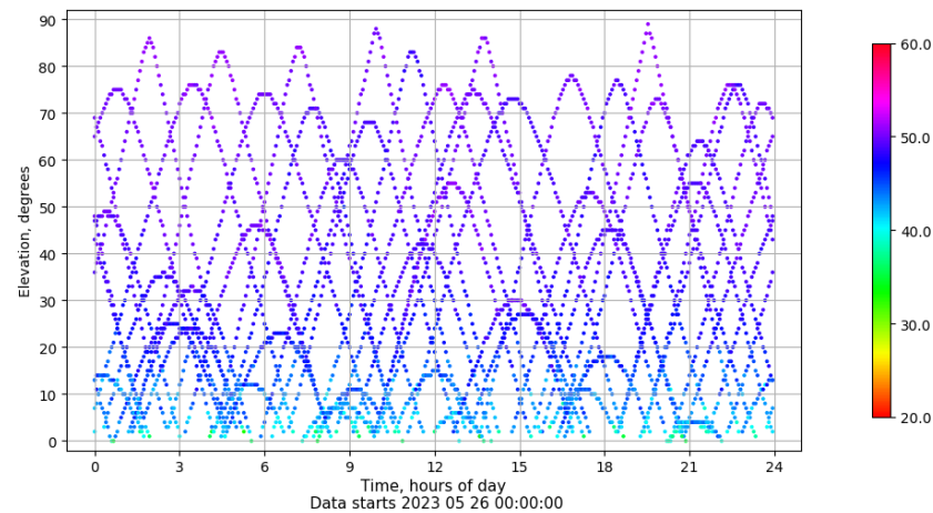
Time-elevation plot for station RIO1. Signal to Noise S1C Data file RIO100ESP_R_2023146.xtr
