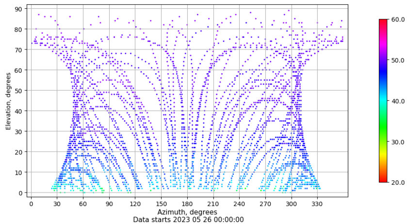
Azimuth-elevation plot for station RIO1. Signal to Noise S1C Data file RIO100ESP_R_2023146.xtr
