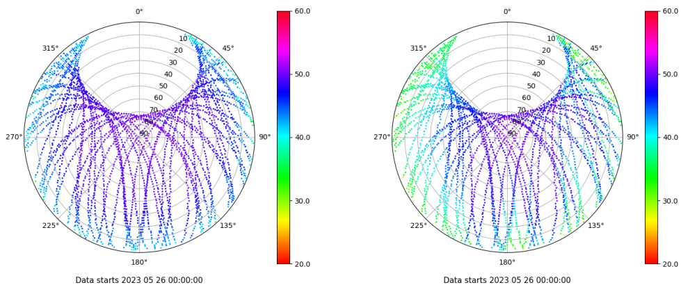
Skyplot for station RIO1. Signal to Noise S1C Data file RIO100ESP_R_2023146.xtr Skyplot for station RIO1. Signal to Noise S2W Data file RIO100ESP_R_2023146.xtr
