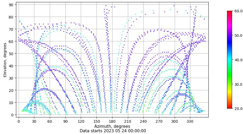
Azimuth-elevation plot for station RIO1. Signal to Noise S1C Data file RIO100ESP_R_2023144.xtr
