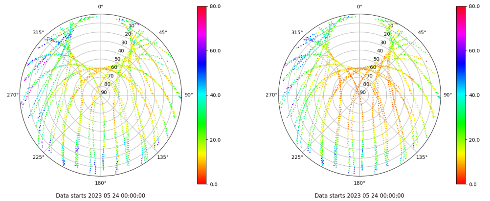
Skyplot for station RIO1. Parameter M1C Data file RIO100ESP_R_2023144.xtr Skyplot for station RIO1. Parameter M2P Data file RIO100ESP_R_2023144.xtr
