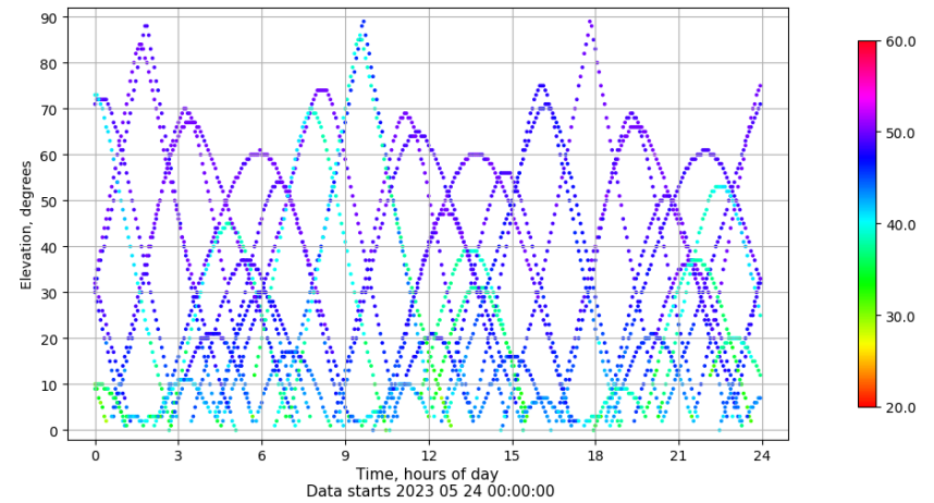
Time-elevation plot for station RIO1. Signal to Noise S1C Data file RIO100ESP_R_2023144.xtr
