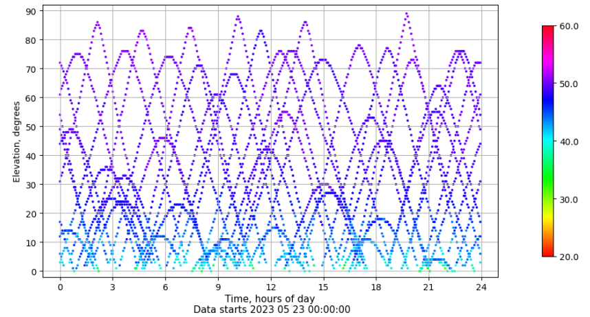
Time-elevation plot for station RIO1. Signal to Noise S1C Data file RIO100ESP_R_2023143.xtr
