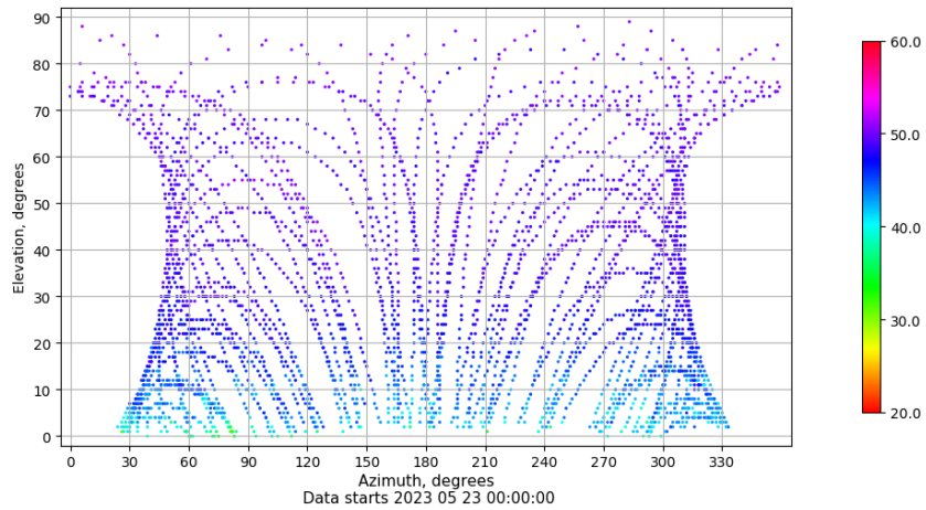
Azimuth-elevation plot for station RIO1. Signal to Noise S1C Data file RIO100ESP_R_2023143.xtr
