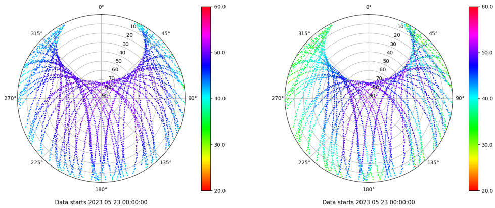
Skyplot for station RIO1. Signal to Noise S1C Data file RIO100ESP_R_2023143.xtr Skyplot for station RIO1. Signal to Noise S2W Data file RIO100ESP_R_2023143.xtr
