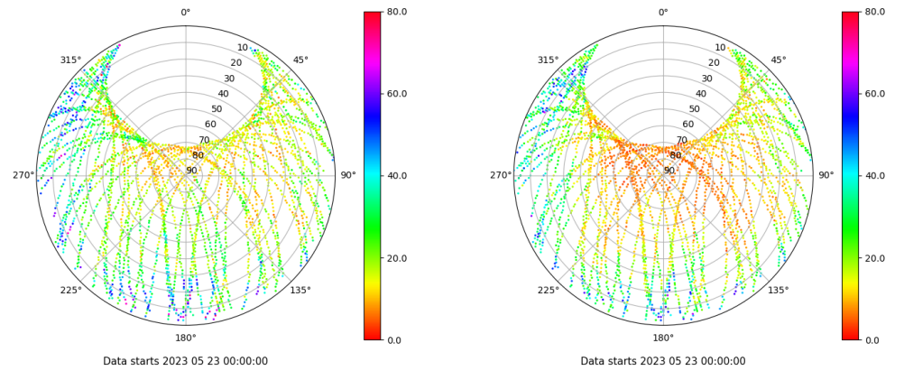
Skyplot for station RIO1. Parameter M1C Data file RIO100ESP_R_2023143.xtr Skyplot for station RIO1. Parameter M2W Data file RIO100ESP_R_2023143.xtr
