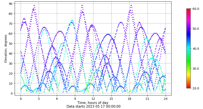
Time-elevation plot for station RIO1. Signal to Noise S1C Data file RIO100ESP_R_2023137.xtr
