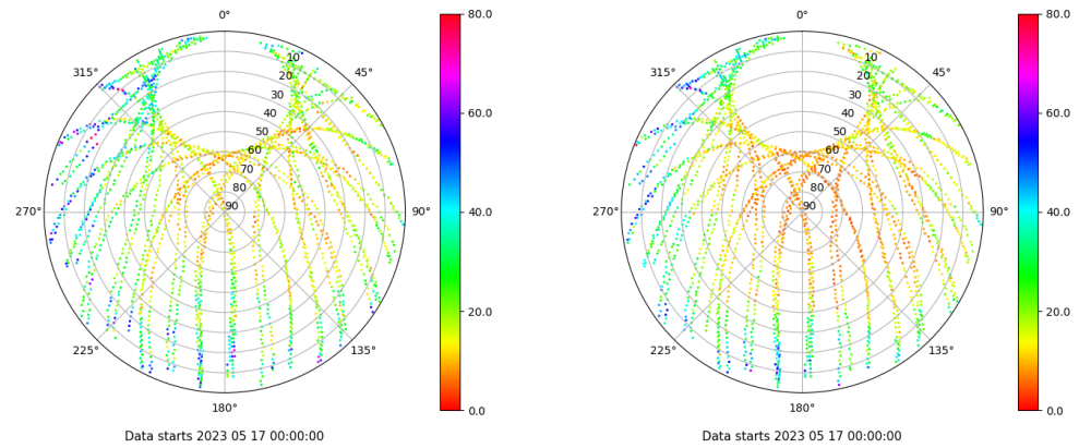
Skyplot for station RIO1. Parameter M1C Data file RIO100ESP_R_2023137.xtr Skyplot for station RIO1. Parameter M2P Data file RIO100ESP_R_2023137.xtr
