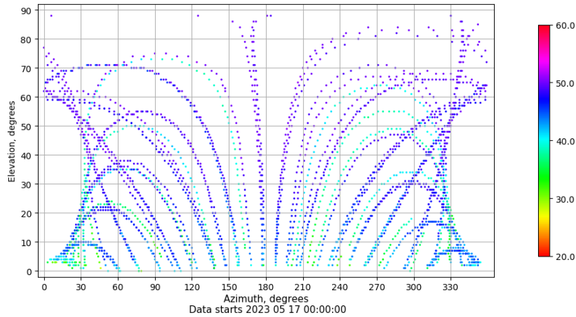
Azimuth-elevation plot for station RIO1. Signal to Noise S1C Data file RIO100ESP_R_2023137.xtr
