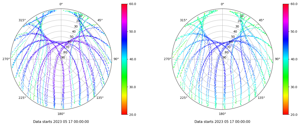
Skyplot for station RIO1. Signal to Noise S1C Data file RIO100ESP_R_2023137.xtr Skyplot for station RIO1. Signal to Noise S2P Data file RIO100ESP_R_2023137.xtr
