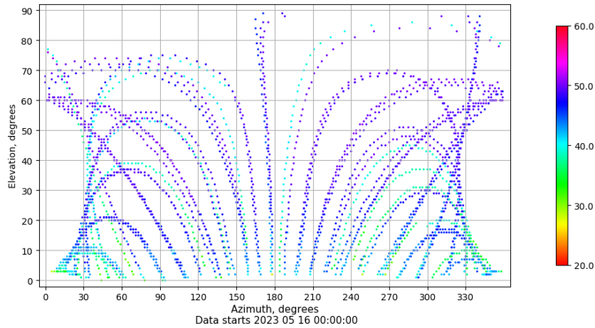
Azimuth-elevation plot for station RIO1. Signal to Noise S1C Data file RIO100ESP_R_2023136.xtr
