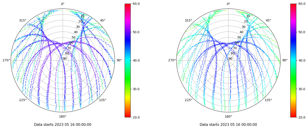
Skyplot for station RIO1. Signal to Noise S1C Data file RIO100ESP_R_2023136.xtr Skyplot for station RIO1. Signal to Noise S2P Data file RIO100ESP_R_2023136.xtr
