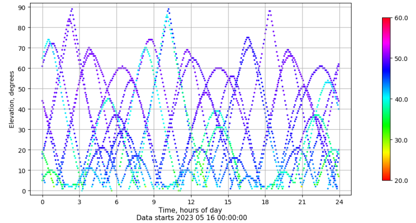
Time-elevation plot for station RIO1. Signal to Noise S1C Data file RIO100ESP_R_2023136.xtr
