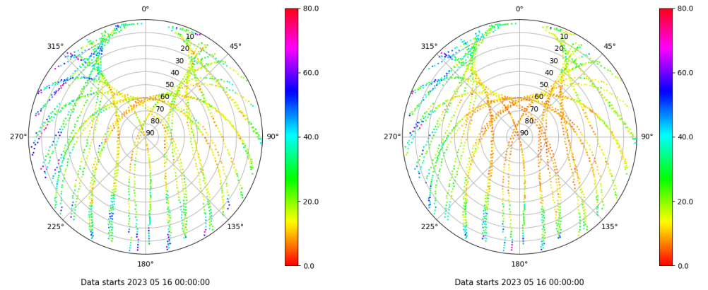
Skyplot for station RIO1. Parameter M1C Data file RIO100ESP_R_2023136.xtr Skyplot for station RIO1. Parameter M2P Data file RIO100ESP_R_2023136.xtr
